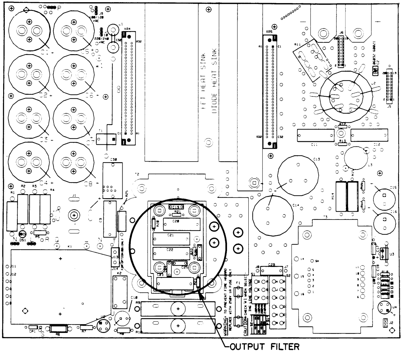
Figure 6-2C. 6032A Main Board (A1) and Output Filter Component Location
