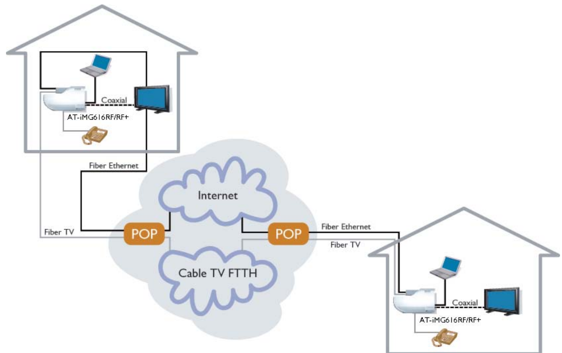
FIGURE 2: LAN CONNECTIONS
