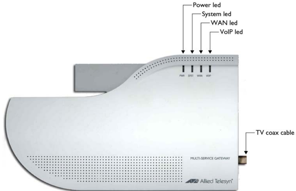
FIGURE 3: TOP VIEW
