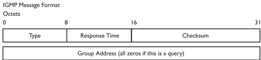
Figure 6- 15. IGMP Message Format
