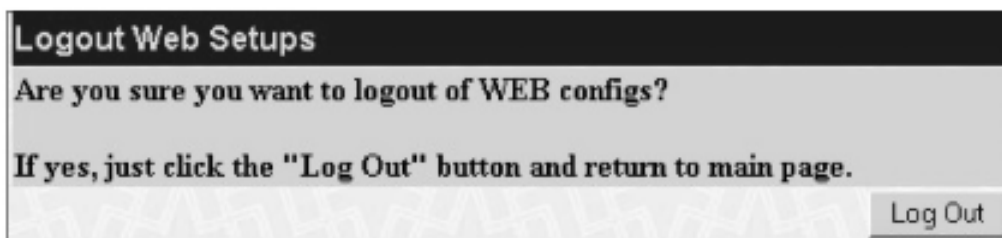
Figure 10- 11 . Logout window
