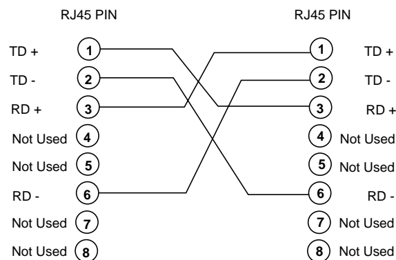
Figure 13 Schematics for Crossover Cable
