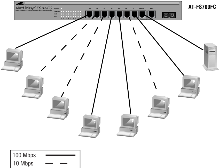
Figure 3 Power Workgroup Topology
