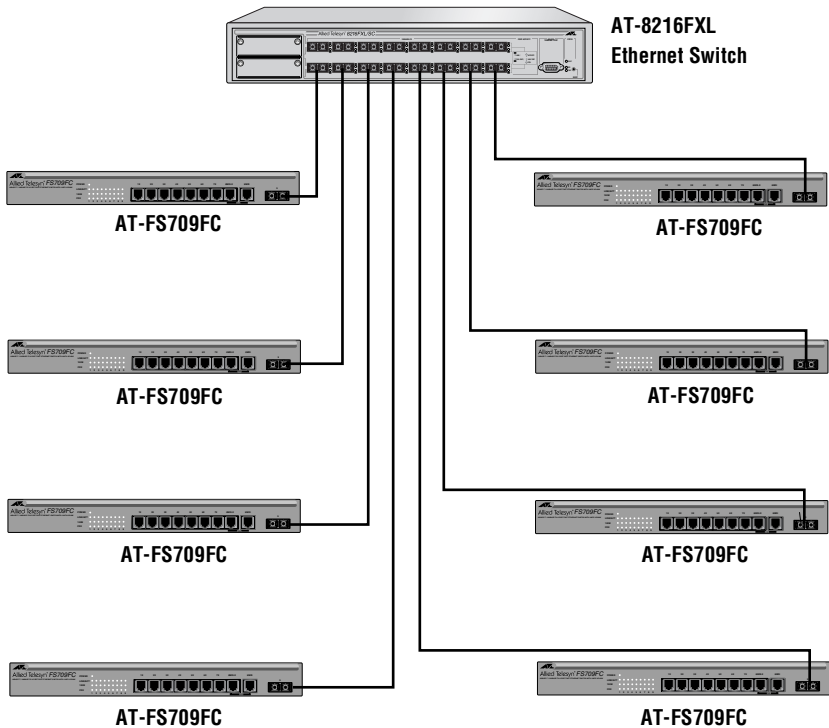
Figure 5 Collapsed Backbone — Switch Topology
