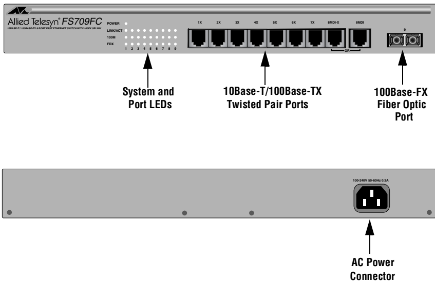
Figure 2 AT-FS709FC Series Fast Ethernet Switch
