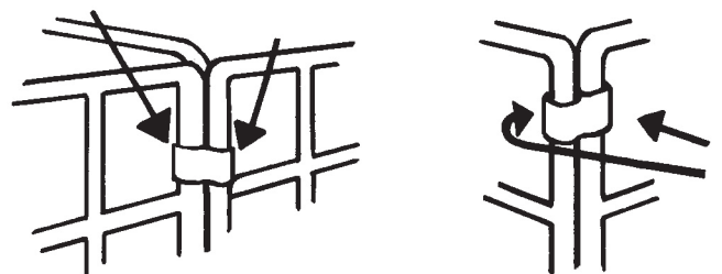
CLIP ATTACHMENT
