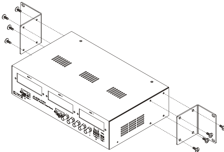
FIG. 6 Installing mounting brackets
