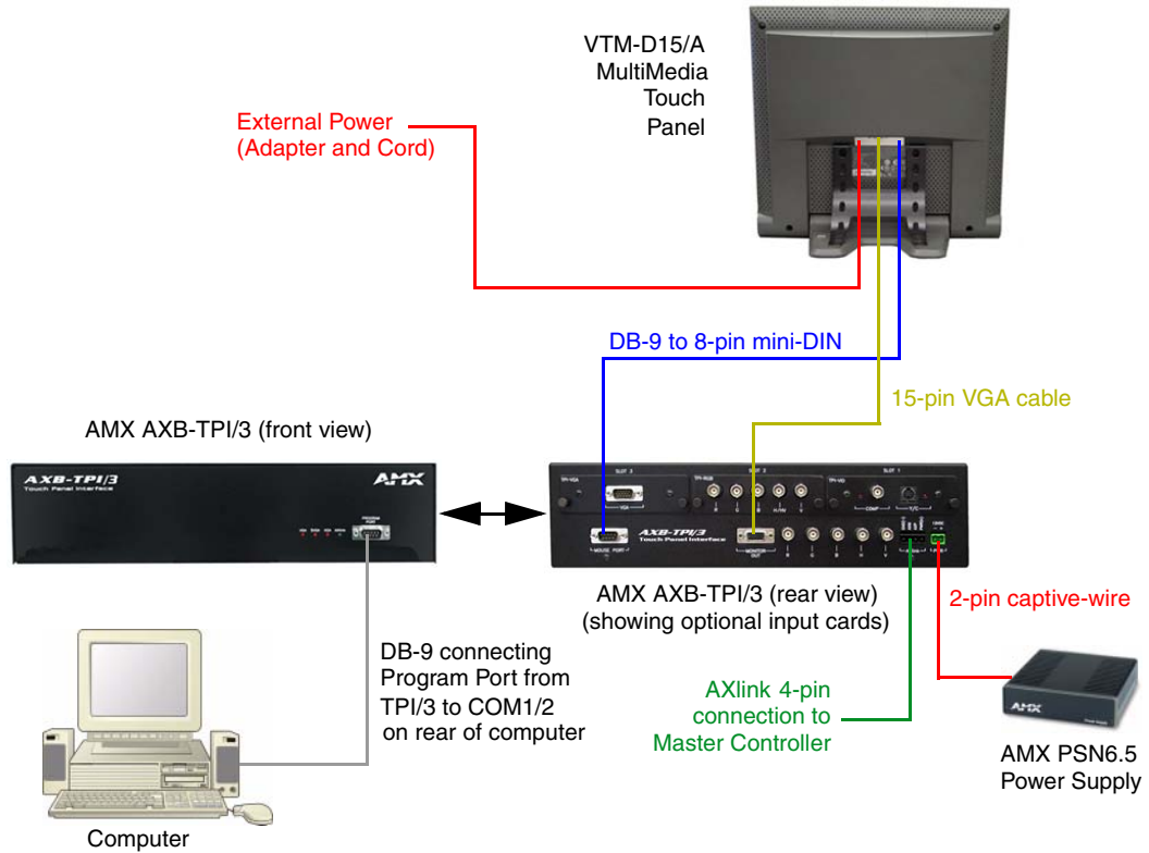
FIG. 4 Sample MultiMedia Touch Panel System Configuration
