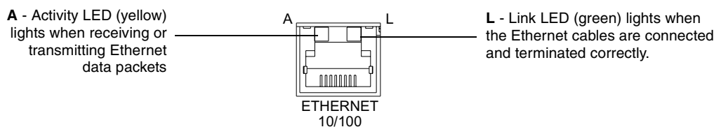
FIG. 49 Layout of Ethernet LEDs
