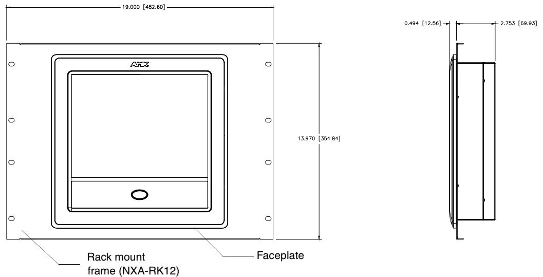
FIG. 46 NXD 12 inch Wall Mount panel installed into an NXA-RK12 Rack Mount Kit
