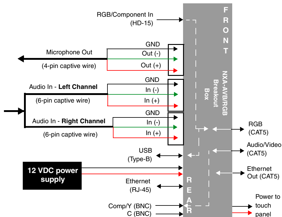
FIG. 4 NXA-AVB/RGB Breakout Box connector wiring diagram
