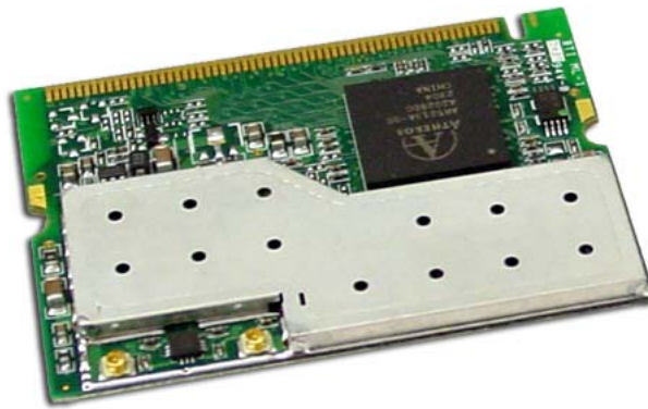
FIG. 13 NXA-PCI80211G mini-PCI Wireless Card
