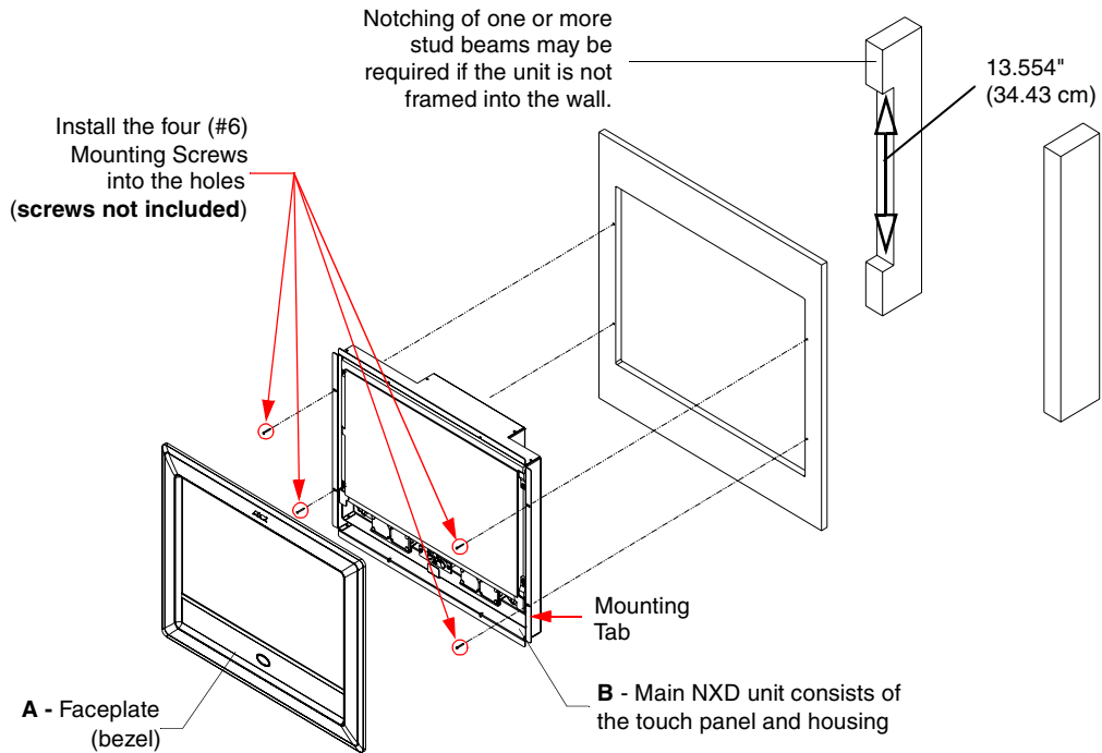
FIG. 62 Wall Mount panel (NXD) installation using screws
