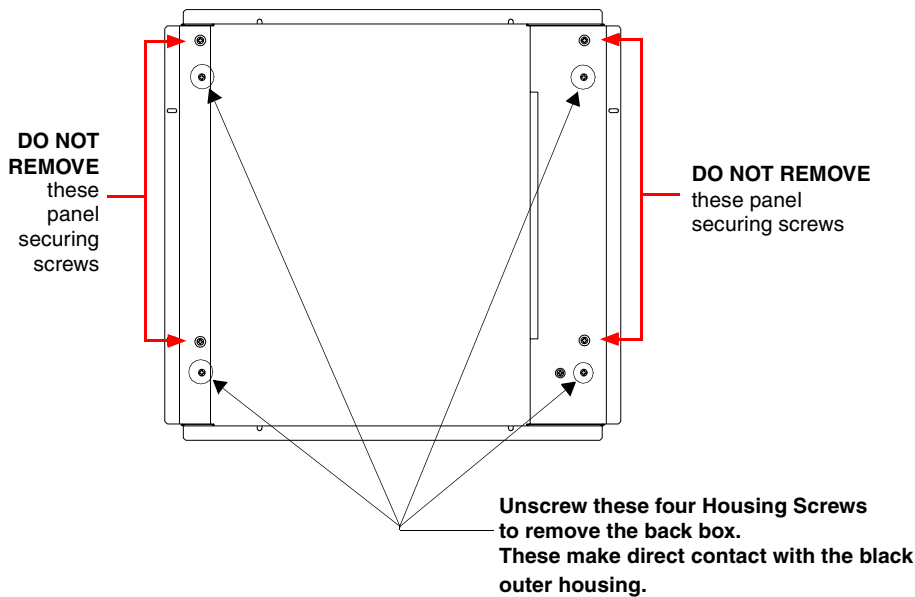
FIG. 33 Location of the attachment screws on the NXD back box
