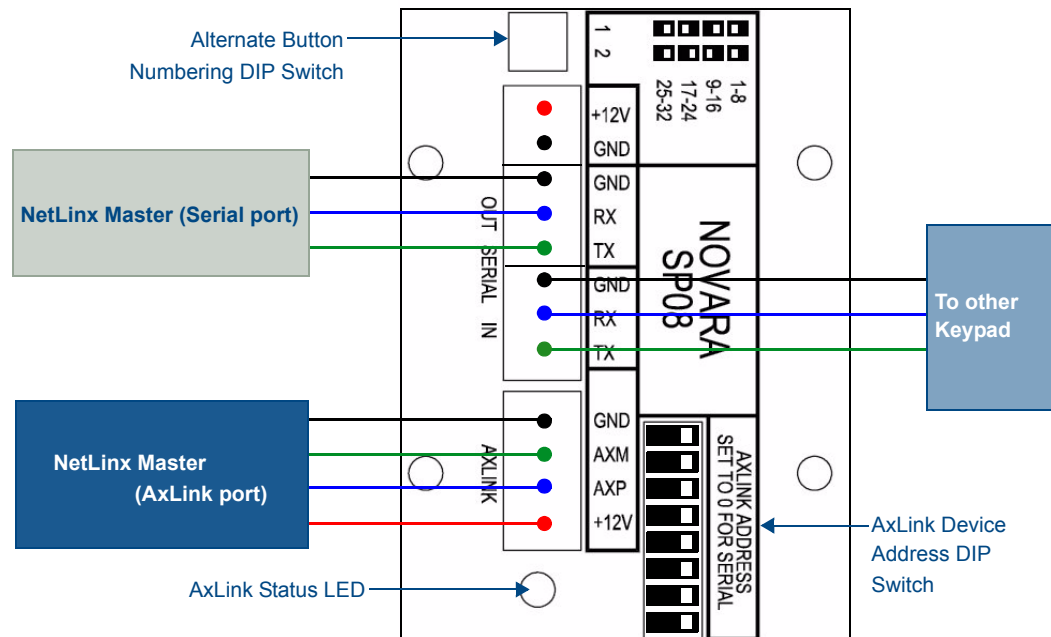
FIG. 7 NOVARA AxLink KeyPads - Rear Panel Connectors
