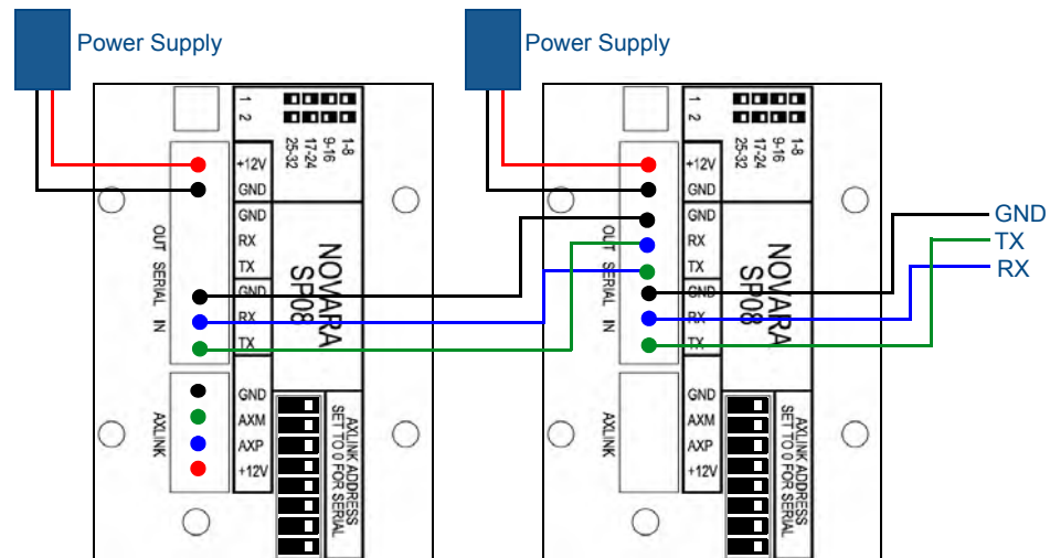
FIG. 10 Daisy-Chaining KeyPads
