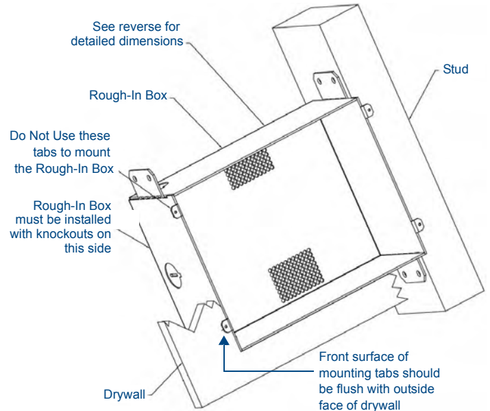
FIG. 1 CB-TP7 - Drywall Installation
