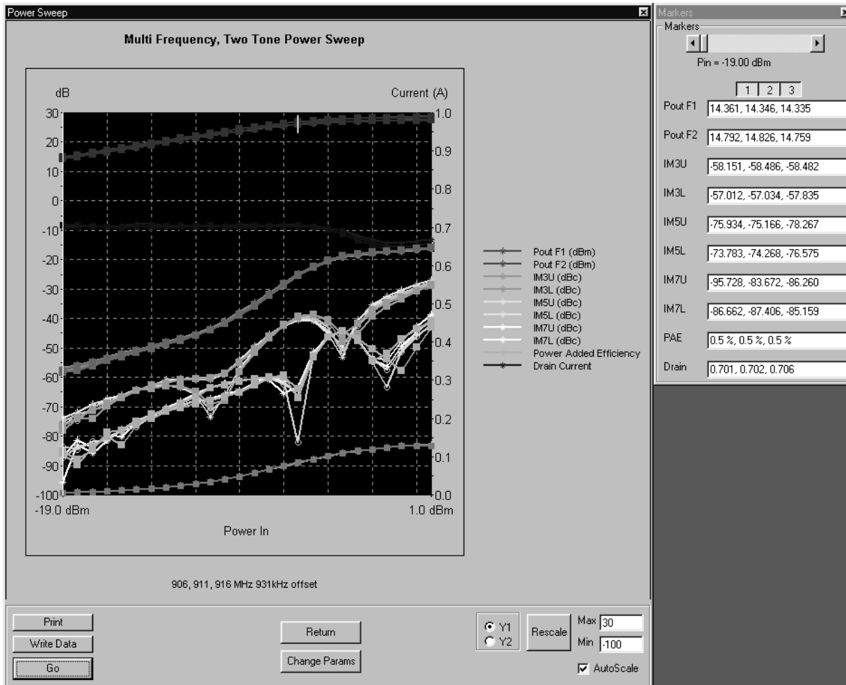
Figure 5-4. Multiple Frequency Power Sweep Test
