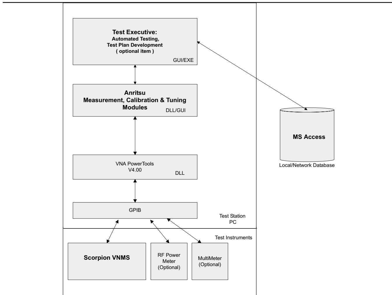
Figure 1-6. PATS Software Structure
