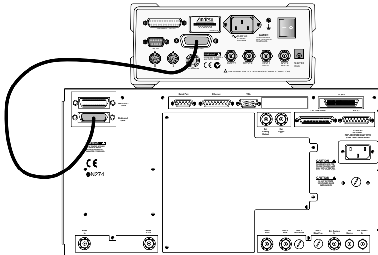
Figure 6-1. ML2430A Series Power Meter GPIB connection to the MS462XX Vector Network Measurement System
