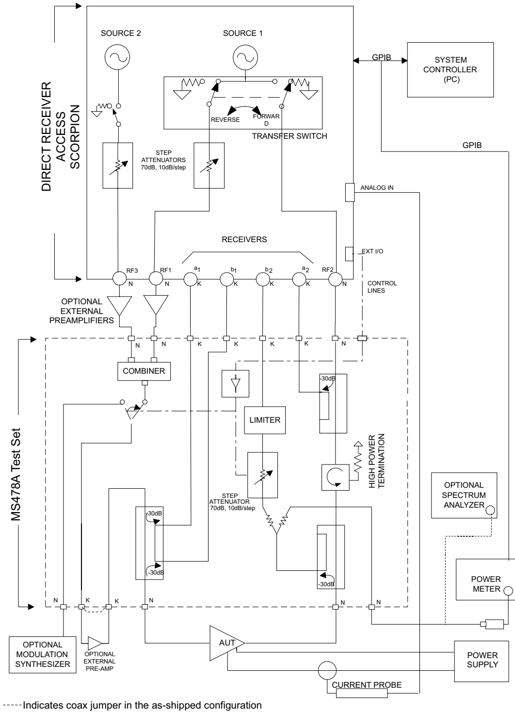
Figure 1-3. Overall Functional Block Diagram of the Option 2 Power Amplifier Test System (PATS) with MS4782A Test Set
