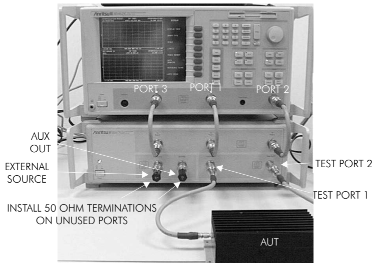
Figure 2-3. ME7840A Front RF Cable Connections (through-line shown between test port 1 and test port 2)
