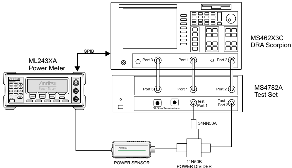
Figure 6-2. Receiver Magnitude Display Linearity Test Setup
