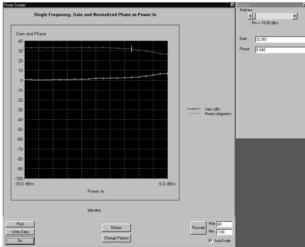
Figure 5-6. Single Frequency Power Sweep Test
