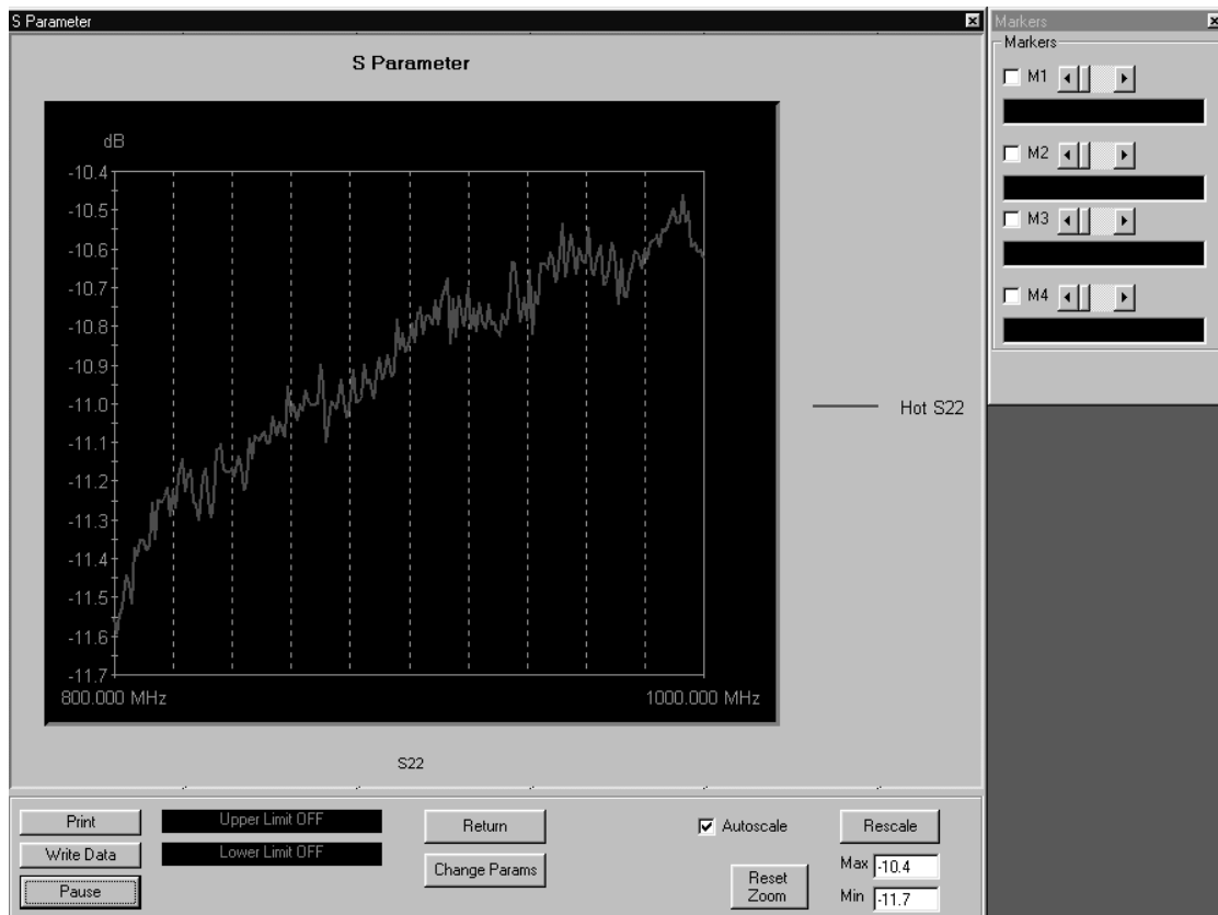
Figure 5-9. Hot S_{22} Test Screen
