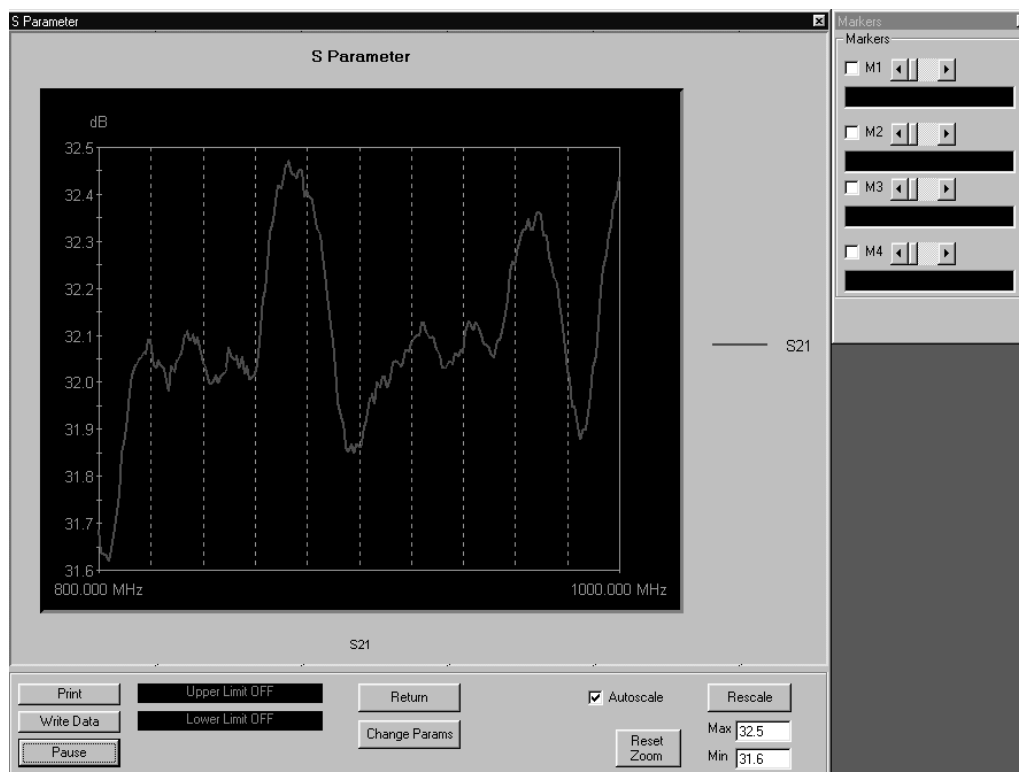
Figure 5-1. S-Parameters Test Screen for S_{21}
