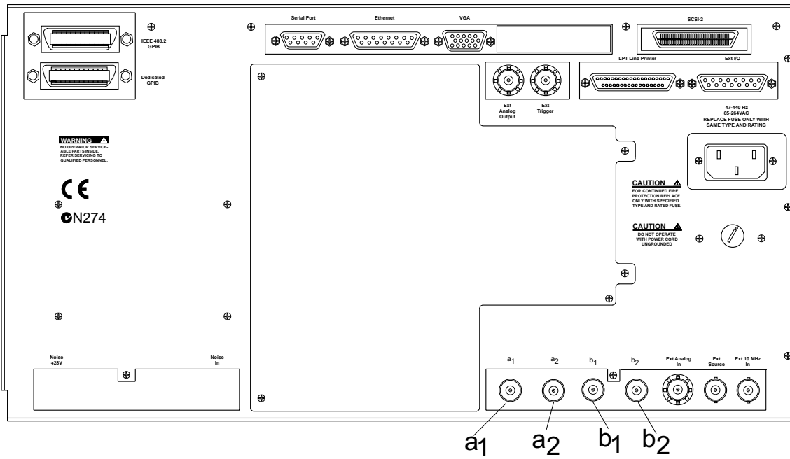
Figure 1-4. MS462XC Rear Panel Showing Ports a 1 , a 2 , b 1 , and b 2
