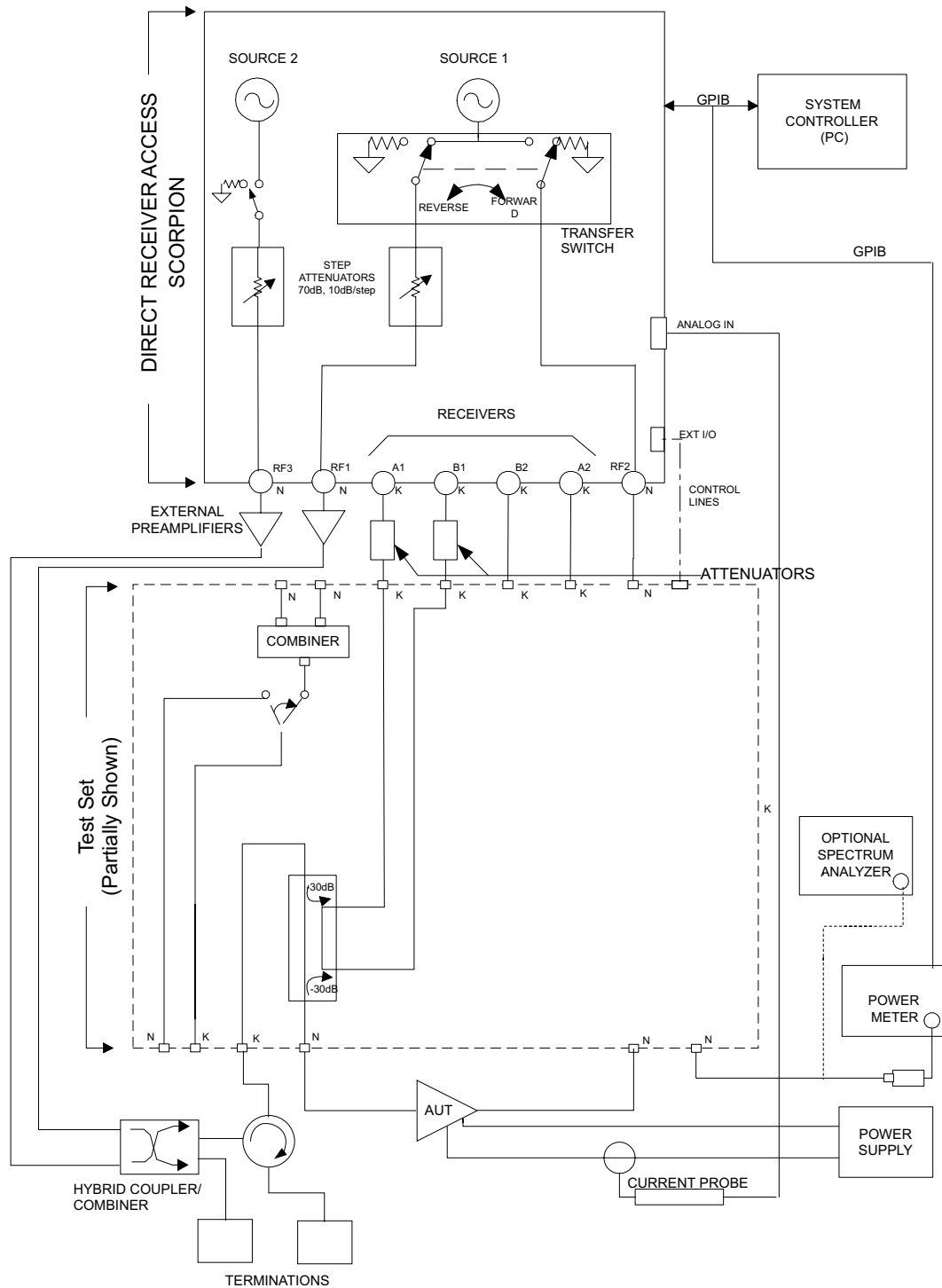
Figure 7-2. MS4782A with External Combiner
