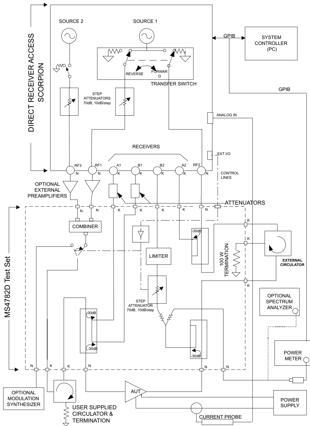
Figure 7-1. MS4782A with External Preamplifiers (Moderate Power)
