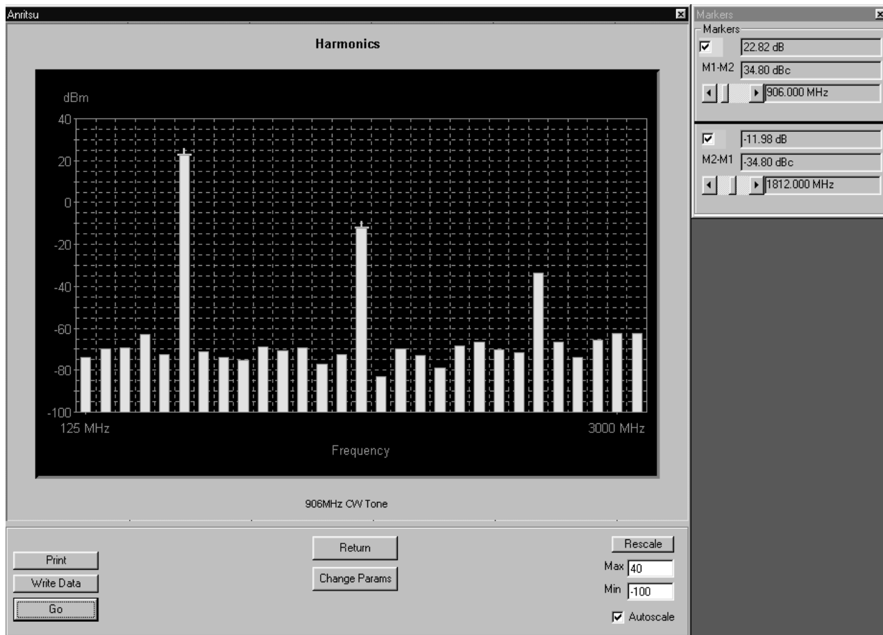
Figure 5-8. Initial Harmonics Test Screen
