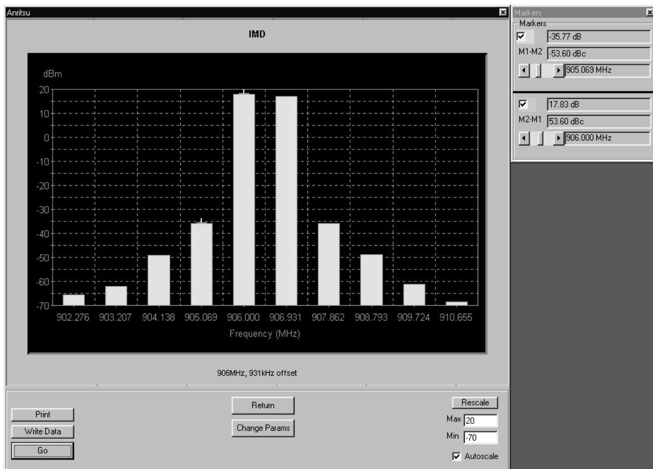
Figure 5-7. Intermodulation Distortion Test Screen
