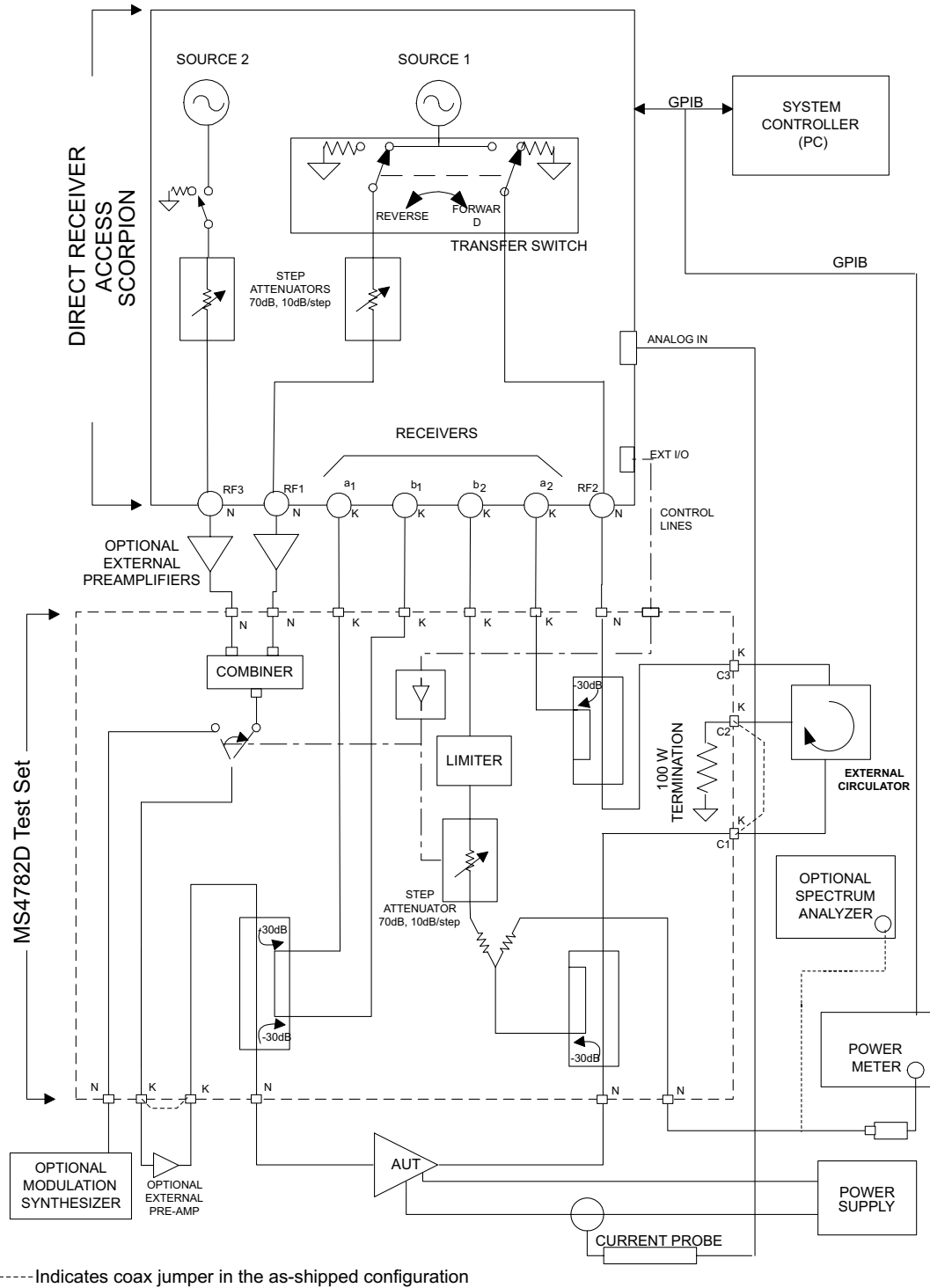
Figure 1-2. Overall Functional Block Diagram of the Basic Power Amplifier Test System (PATS) with MS4782D Test Set
