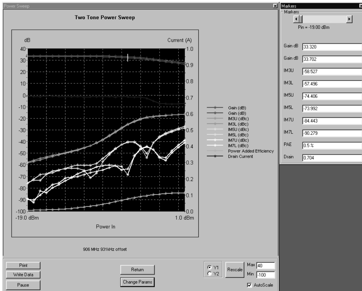
Figure 5-5. Power Sweep Gain and IMD Test Screen, with Markers Selected
