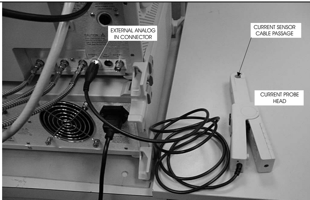
Figure 2-4. Current Probe Connection
