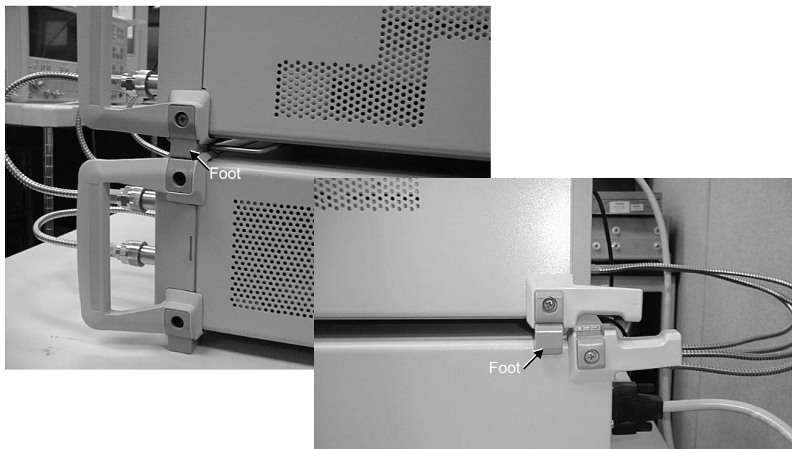
Figure 2-1. ME7840A Component Assembly
