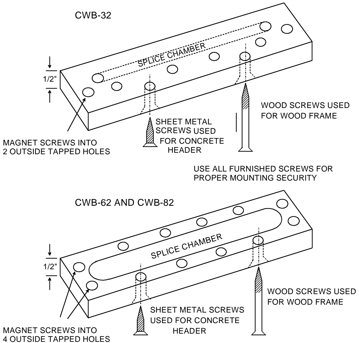
FIG. 12: WOOD FRAME AND CONCRETE HEADER BRACKET
