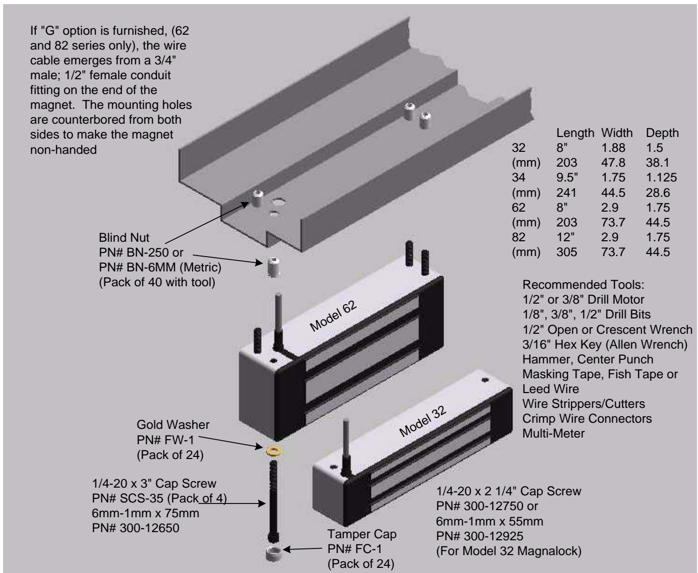
FIG. 2: STANDARD MAGNET DIMENSIONS AND ASSEMBLY
