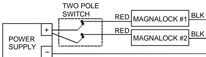
FIG. 17: DOUBLE POLE SWITCHING OF TWO LOCK INSTALLATION
