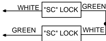
FIG. 16: DOUBLE DOOR WIRING WITH "SC" LOCKS
