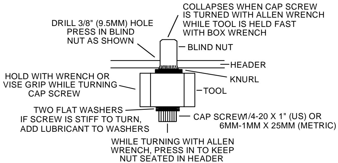
FIG. 4: COLLAPSING THE BLIND NUTS
