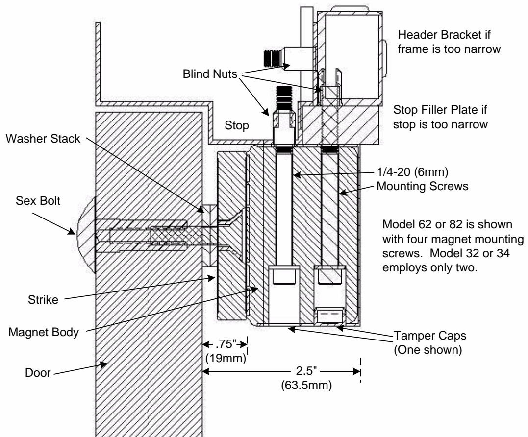
FIG. 5: TYPICAL MOUNTING ON OUTSWINGING DOOR
