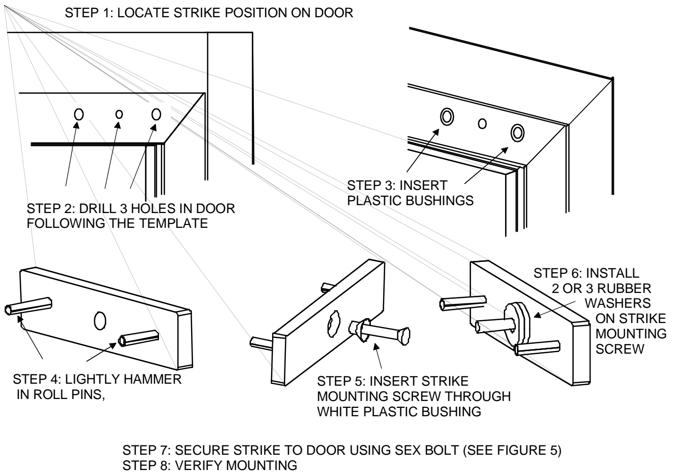
FIG. 1: STEPS IN MOUNTING THE STRIKE
