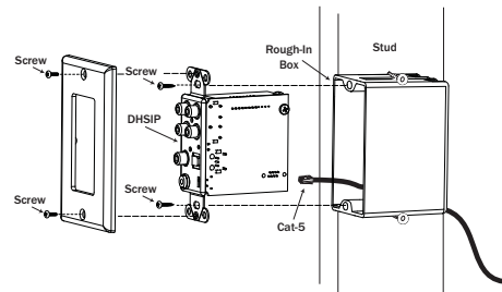
Figure 2.2: Installing the DHSIP
