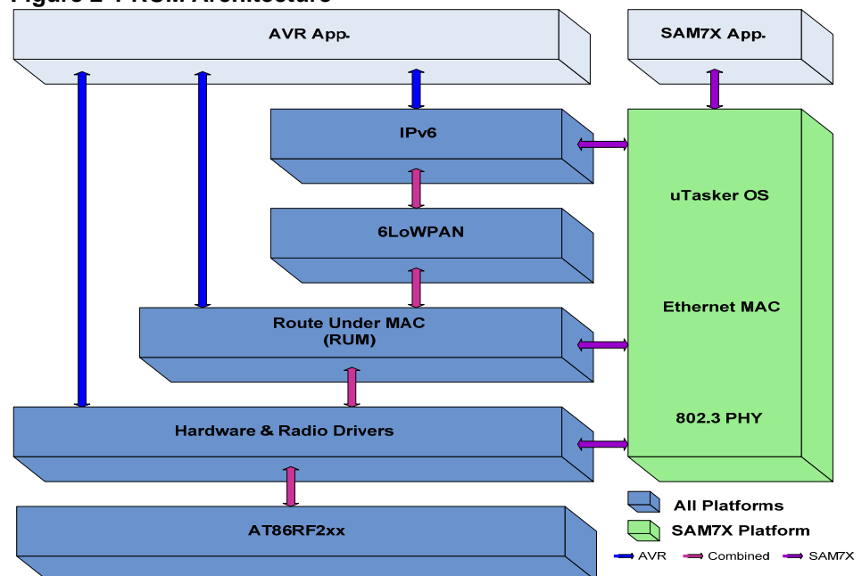
Figure 2-1 RUM Architecture
