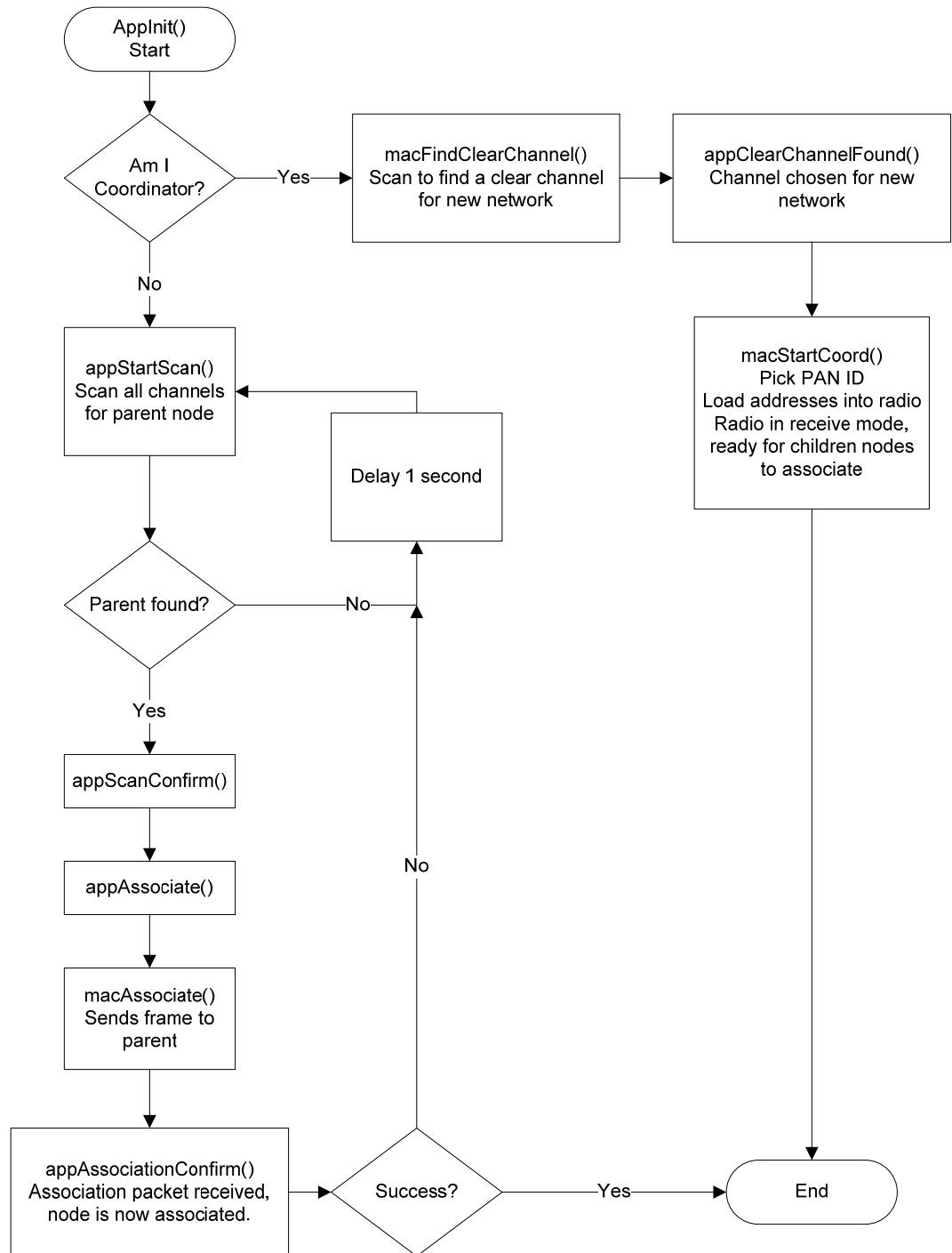
Figure B-2 applnit overview
