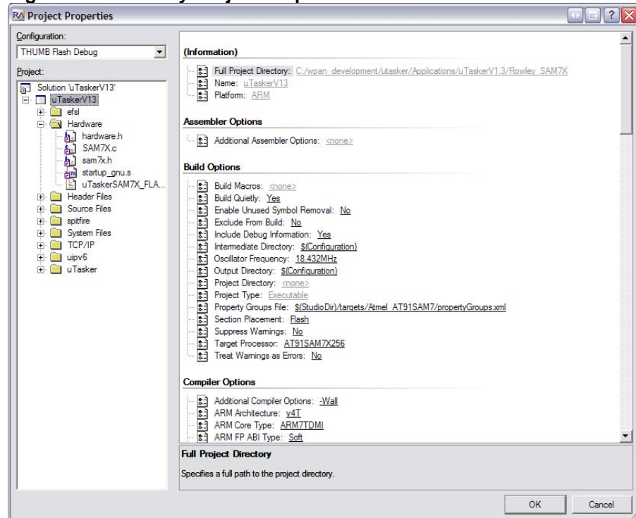
Figure D-2-3 Rowley Project Properties
