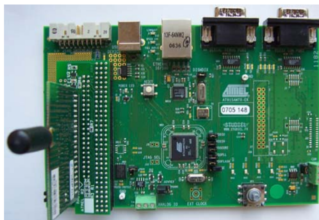
Figure E-1-3 AT91SAM7X-EK with REB/REX_ARM Connected
