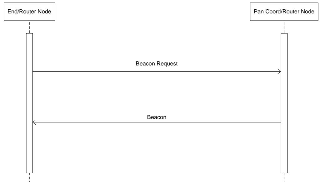
Figure A-4-1 Channel Scan Message Sequence
