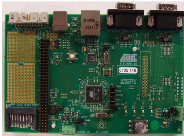
Figure E-1-1 AT91SAM7X-EK Standard Board
