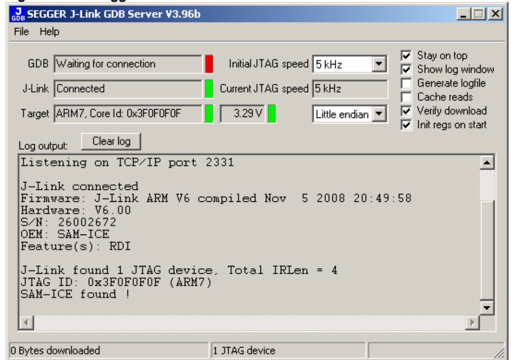
Figure D-3-11 Segger J-Link Connection Screen
