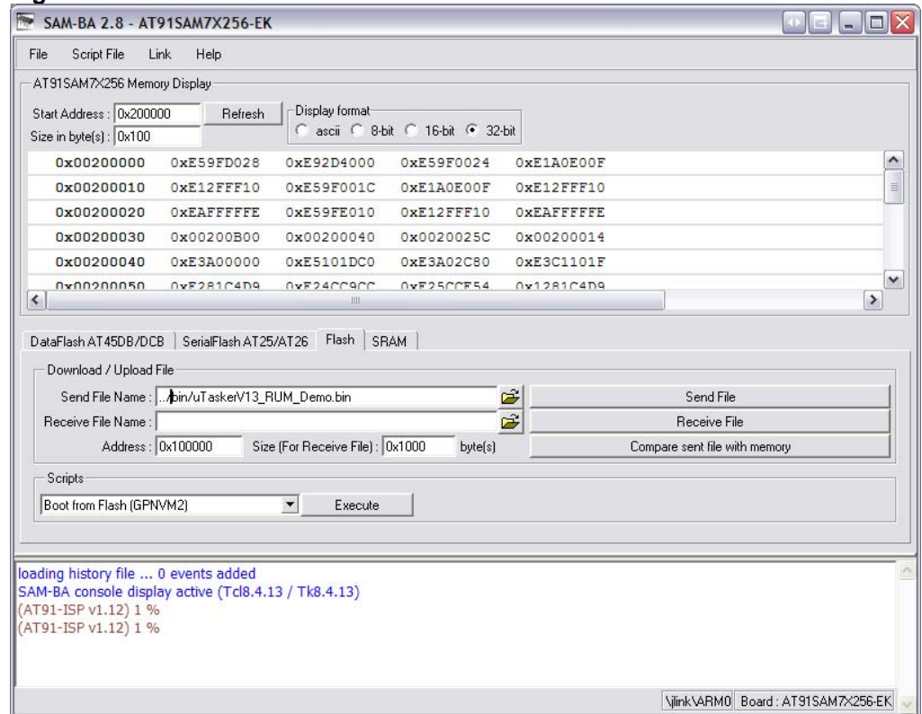
Figure 4-6-2 SAM-BA File Selection
