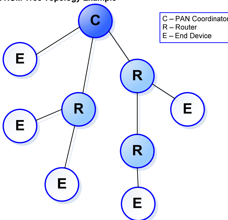
Figure 2-2 RUM Tree Topology Example
