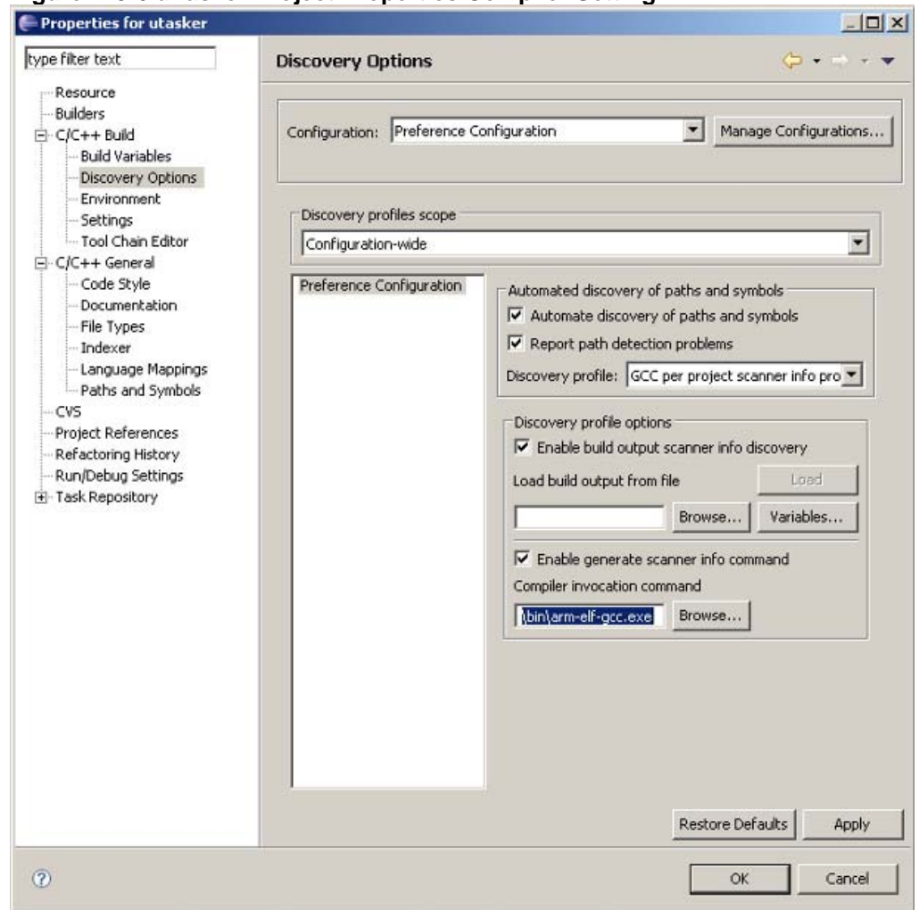
Figure D-3-6 uTasker Project Properties Compiler Setting
