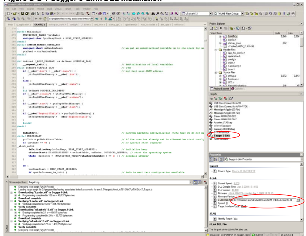
Figure D-2-1 Segger J-Link DLL Installation
