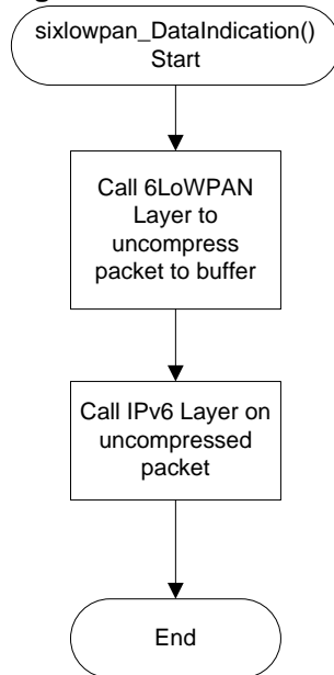
Figure B-8 ARM 6LoWPAN DataIndication
