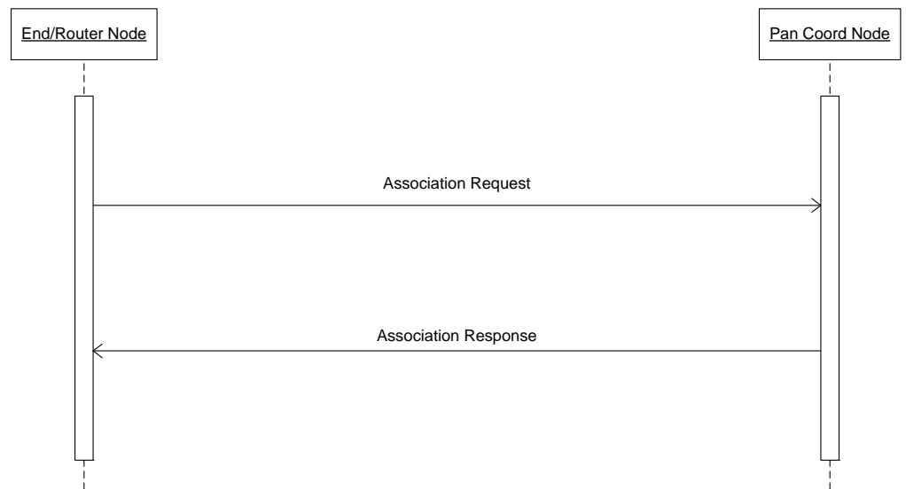
Figure A-4-2 Direct Association Message Sequence
