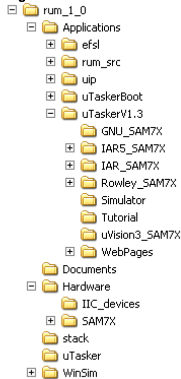
Figure D-1-3 uTasker and RUM Integrated Folder Structure
