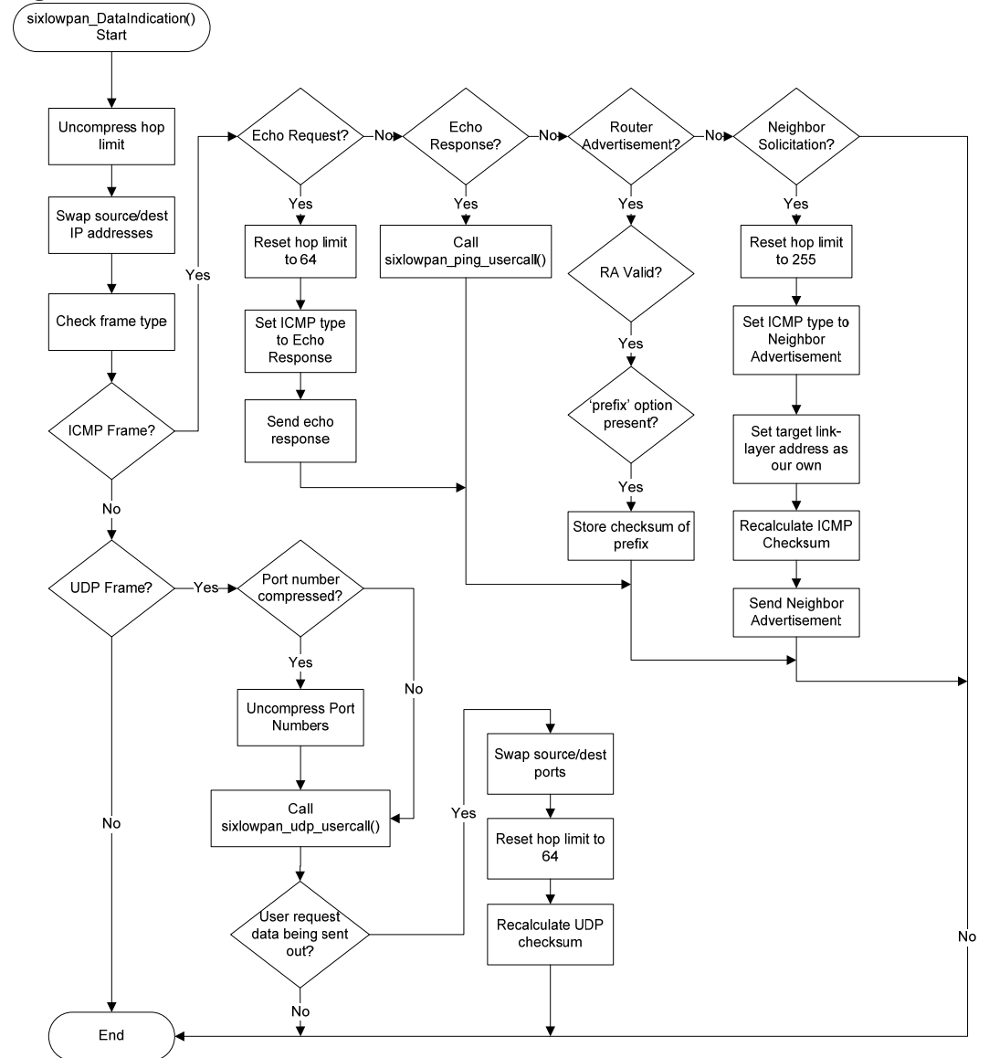
Figure B-7 AVR 6LoWPAN DataIndication
