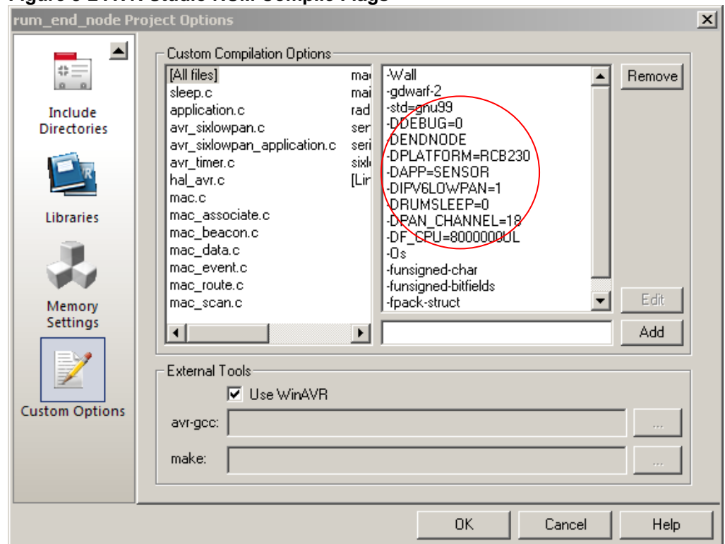
Figure 3-2 AVR Studio RUM Compile Flags
