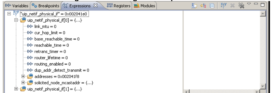
Figure D-3-18 Debug Watch Expressions
