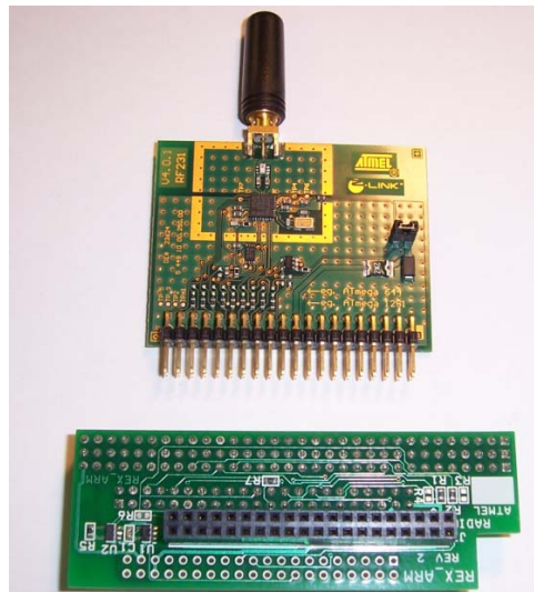
Figure E-1-2 REB and REX_ARM adaptor
