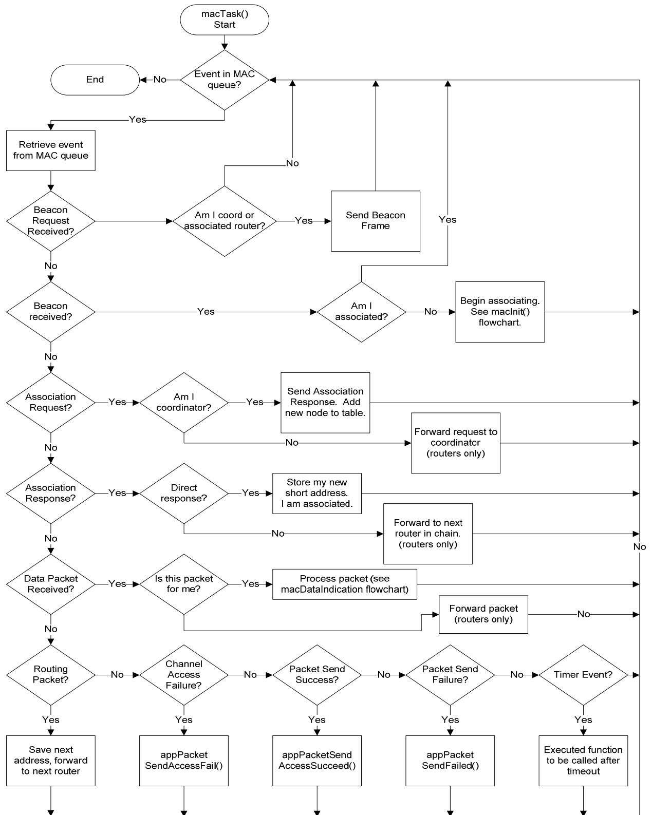
Figure B-3 macTask overview
