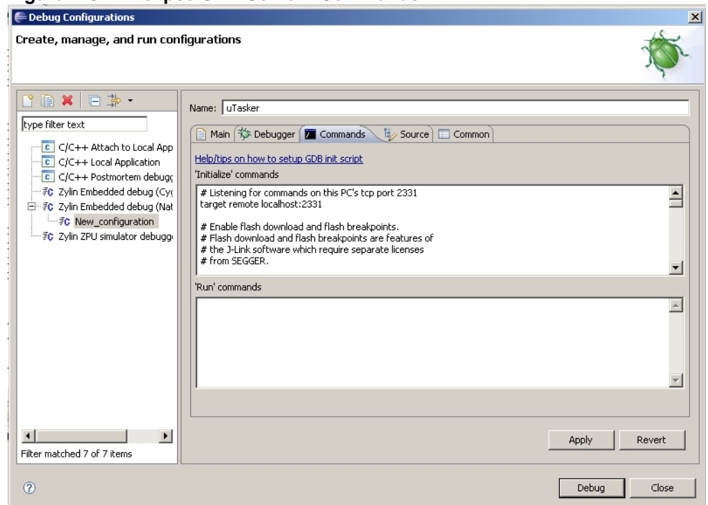
Figure D-3-14 Eclipse GDB Server - Commands
