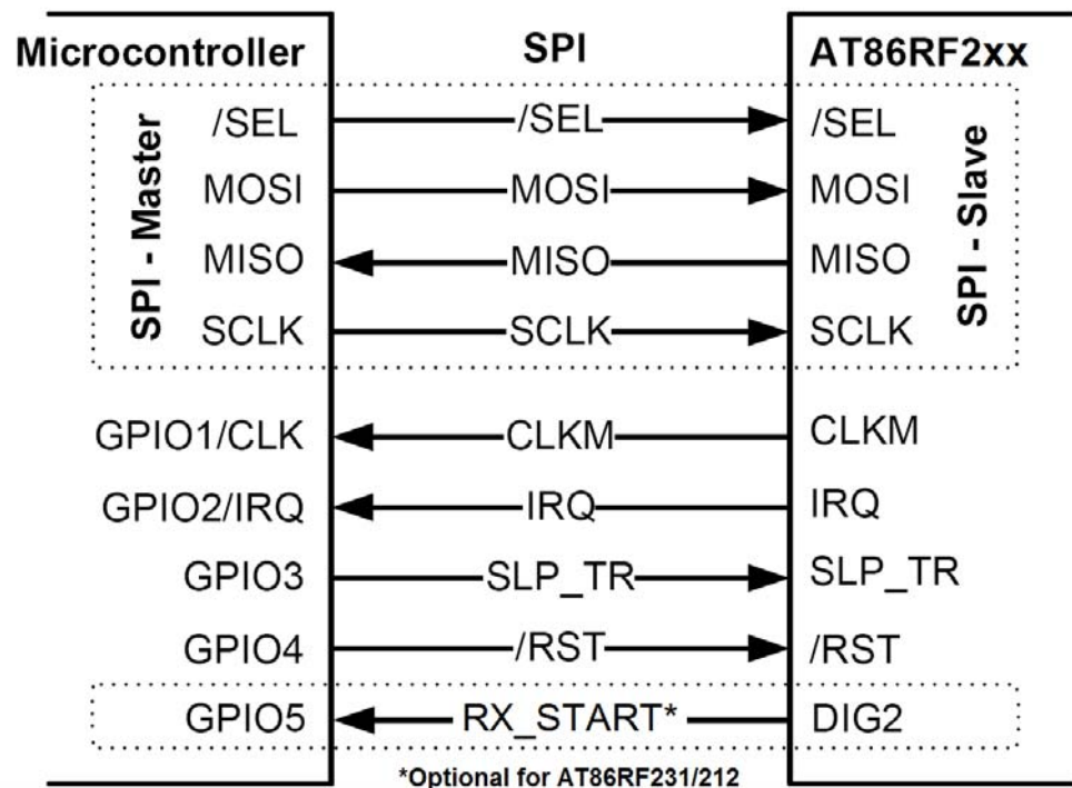
Figure 4-2-1 Microcontroller to Transceiver Connections
