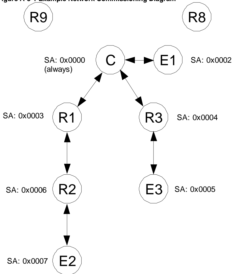
Figure A-5-1 Example Network Commissioning Diagram
