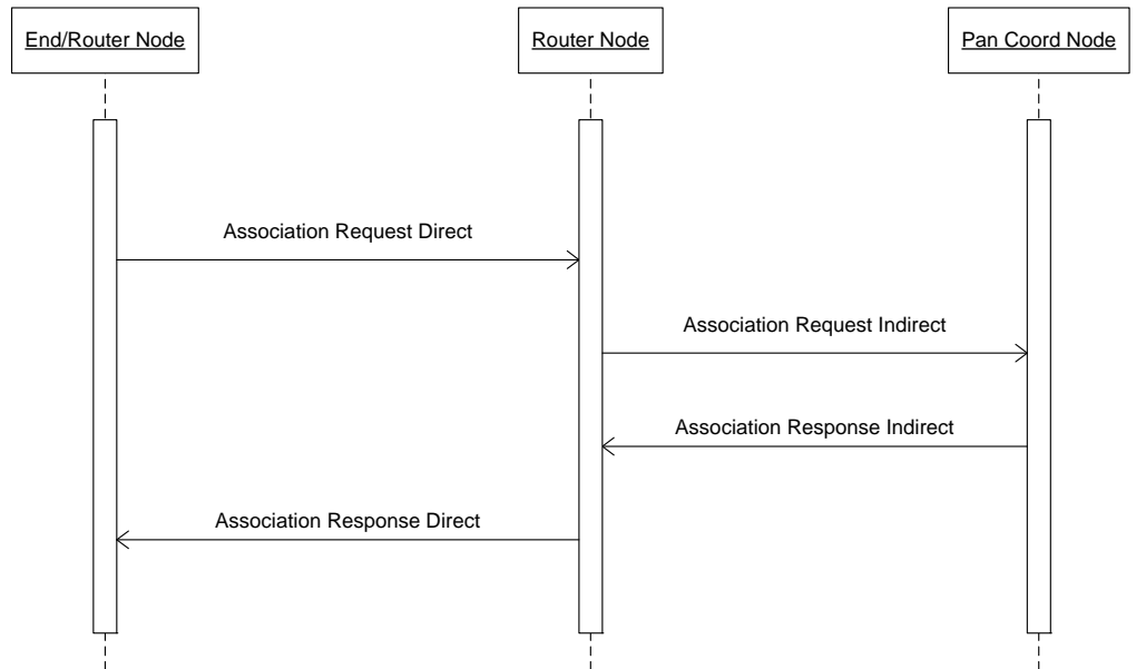
Figure A-4-3 In-Direct Association Message Sequence
