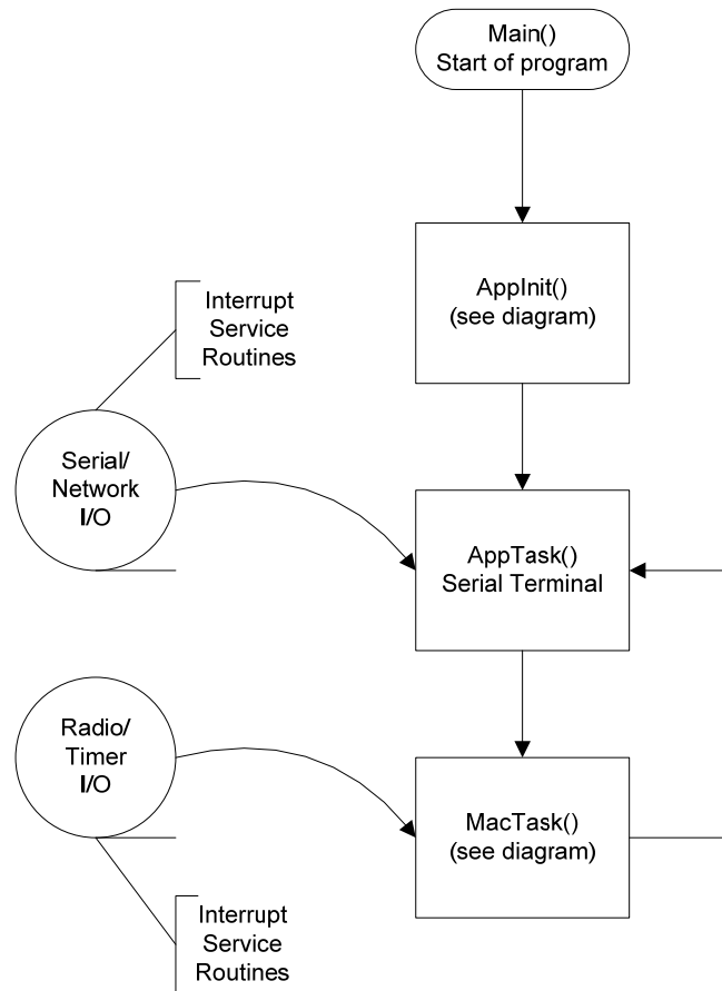
Figure B-1 Overall Program Structure.
