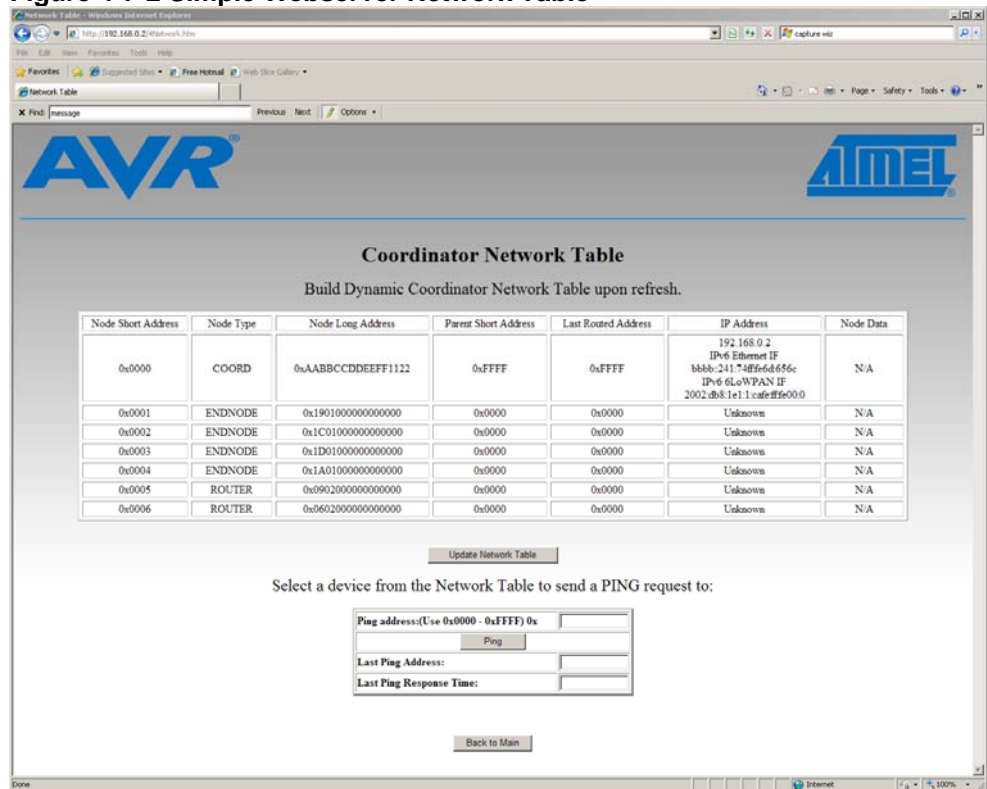
Figure 4-7-2 Simple Webserver Network Table
