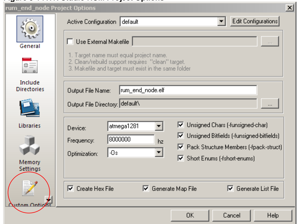
Figure 3-1 AVR Studio RUM Project Options
