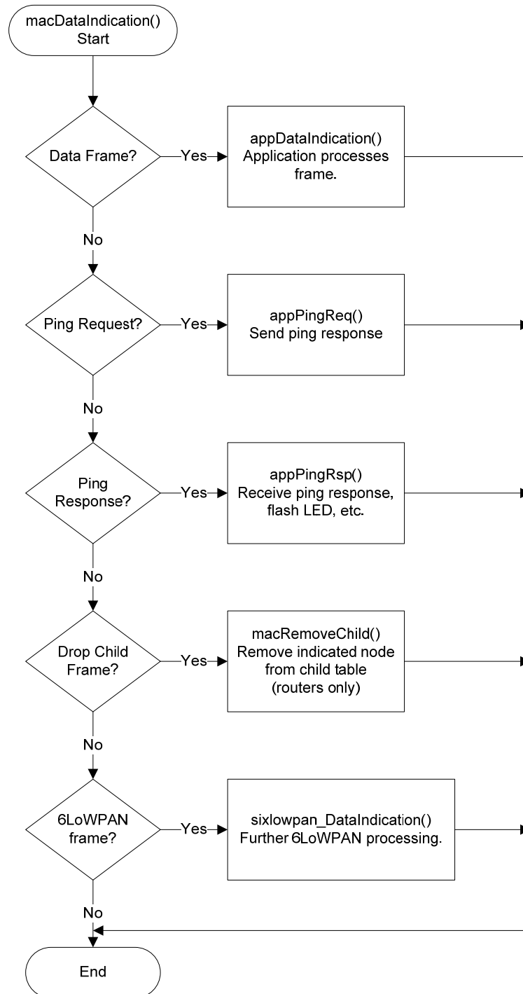
Figure B-4 macDataIndication overview
