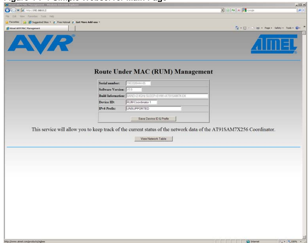
Figure 4-7-1 Simple Webserver Main Page
