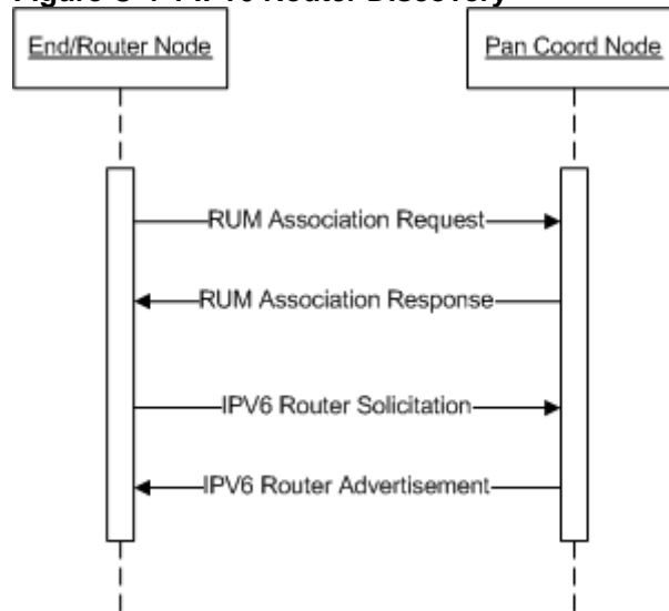
Figure C-4-1 IPv6 Router Discovery
