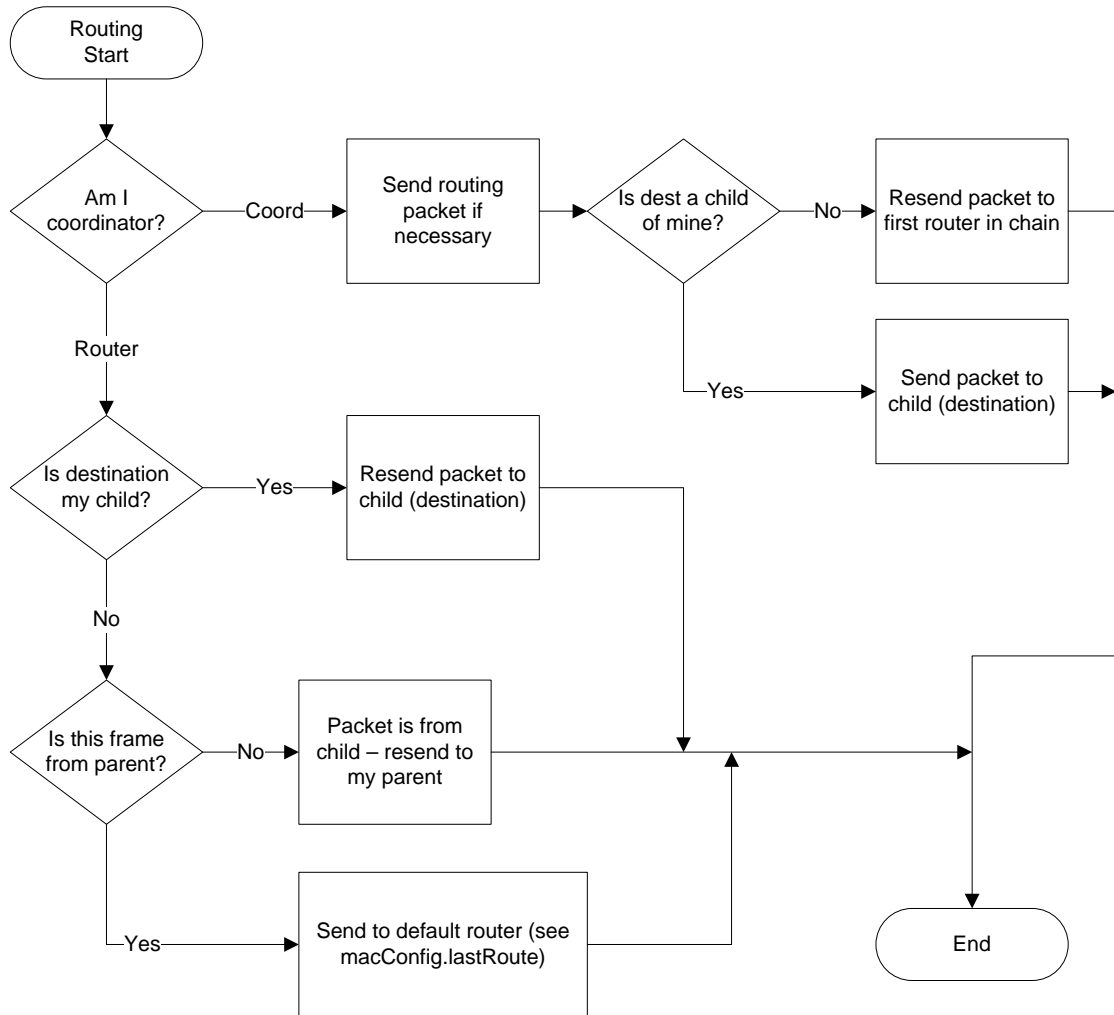
Figure B-5 Frame routing overview
