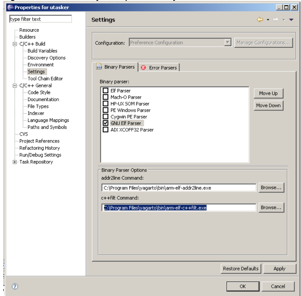
Figure D-3-7 uTasker Project Properties Binary Parser
