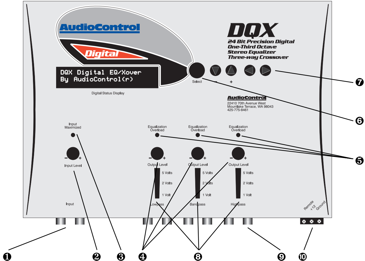
Figure 2: Top view of DQX
