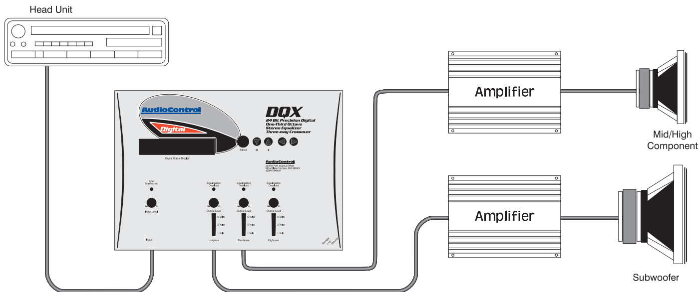
Figure 4: DQX in a two-way system
