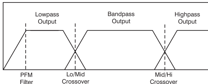
Figure 10: Crossover Response Curve
