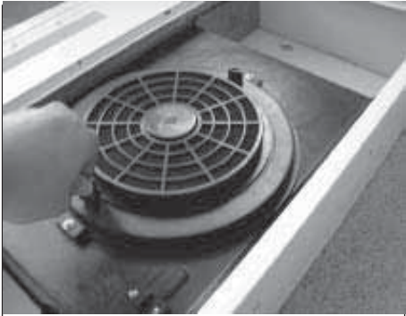
1. Pull up and twist the two spring loaded clips around the carbon filter holder.
