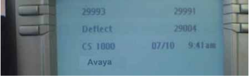
Figure 7: Call deflect
