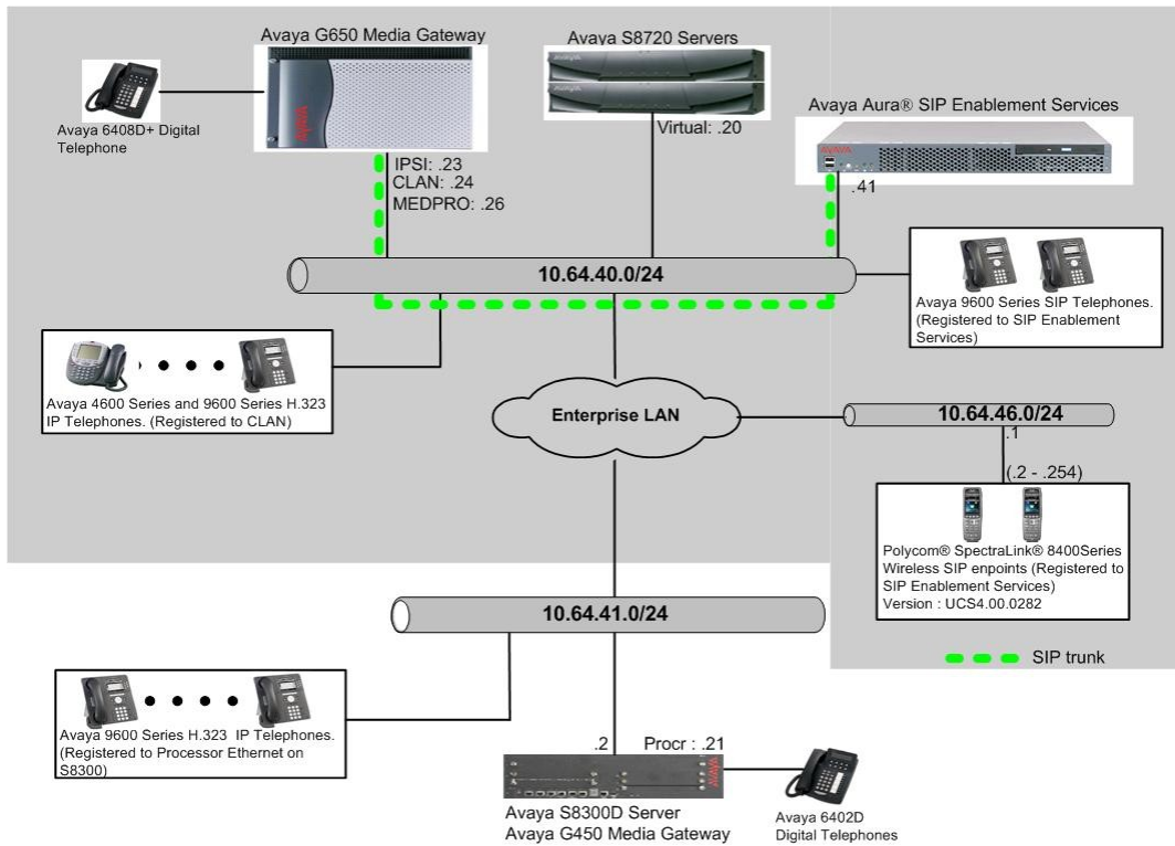
Figure 1: Test Configuration of SpectraLink 8400 Series
