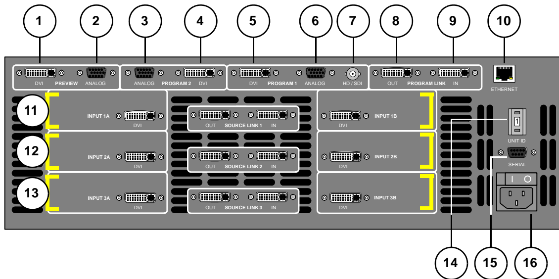
Figure 3. VPx Rear Panel
