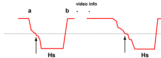
Image 11-11 Hs horizontal sync pulse a active low b active high
