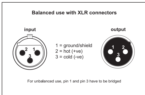
Fig. 4.3: XLR connectors
