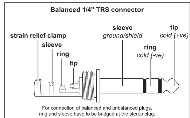
Fig. 4.5: 1/4" TRS connector
