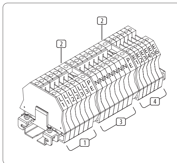
Illustration: LD6230 connector terminal strip
