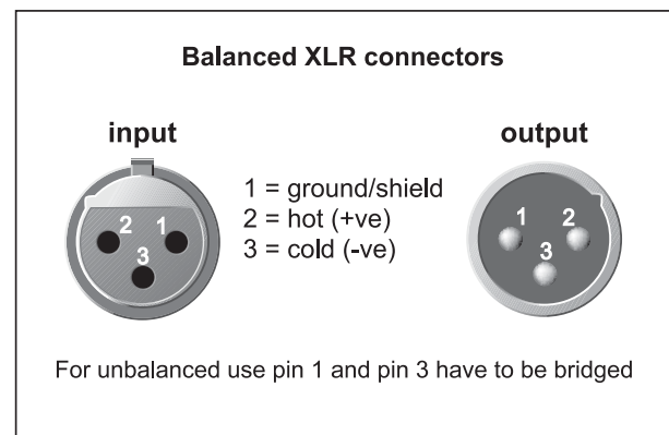
Fig. 5.1: XLR connectors
