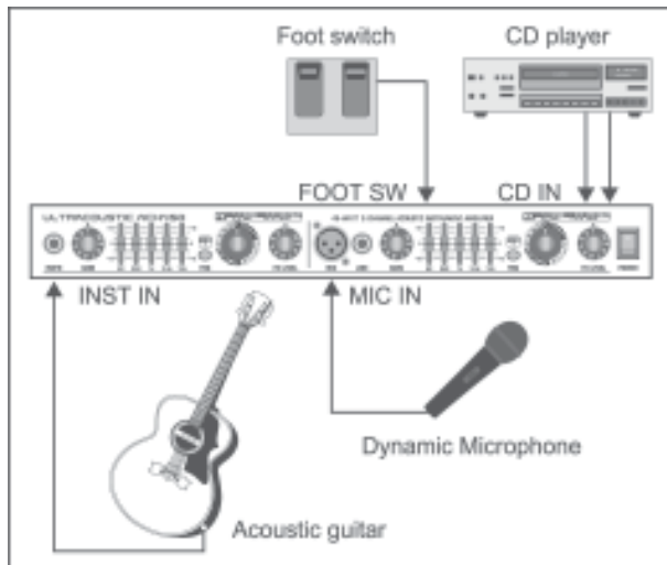
Fig. 3.1: Cabling options of the ACX450
