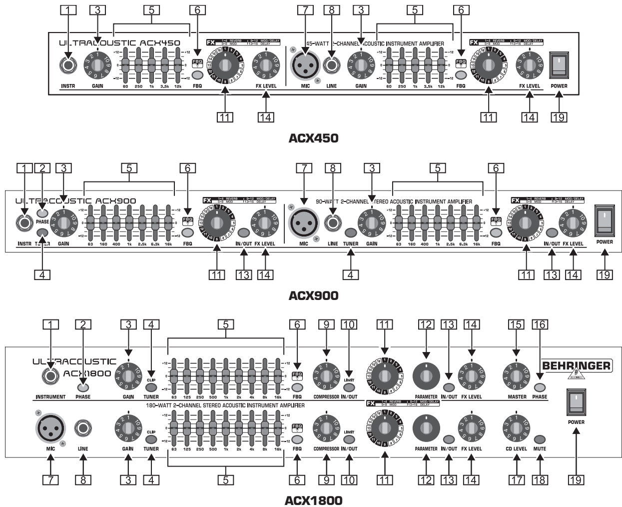
Fig. 2.1: The front panel control elements
