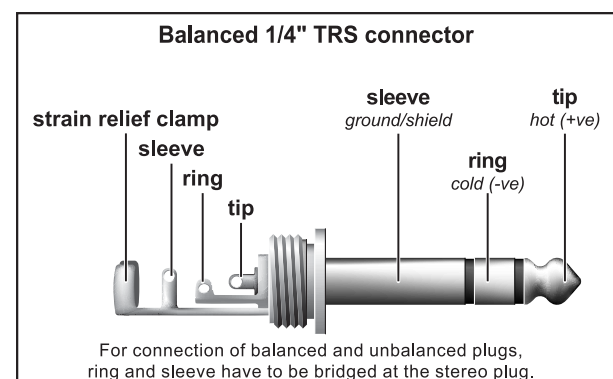
Fig. 5.2: 1/4" stereo TRS connector
