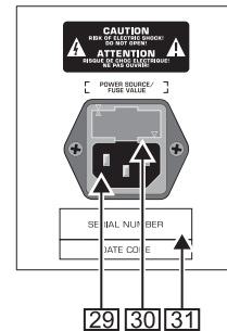
Fig. 2.3: Standard IEC power receptacle, fuse holder and serial number (rear panel)
