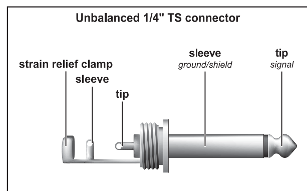
Fig. 5.3: 1/4" TS connector
