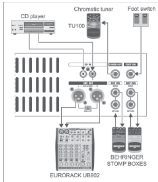
Fig. 3.2: Extended connecting options (ACX900 and ACX1800)
