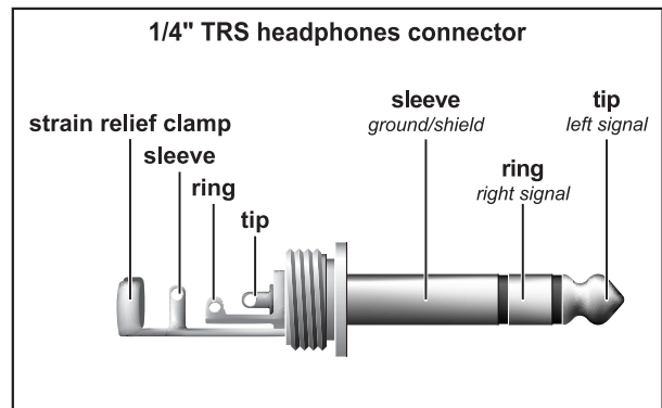
Fig. 8.4: Headphones connector
