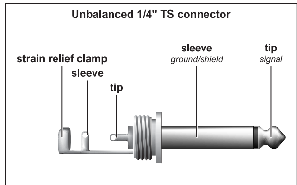
Fig. 8.2: 1/4" TS connector
