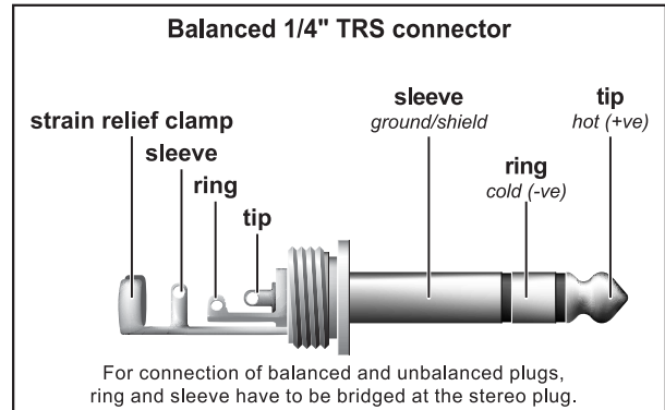
Fig. 8.3: 1/4" TRS connector
