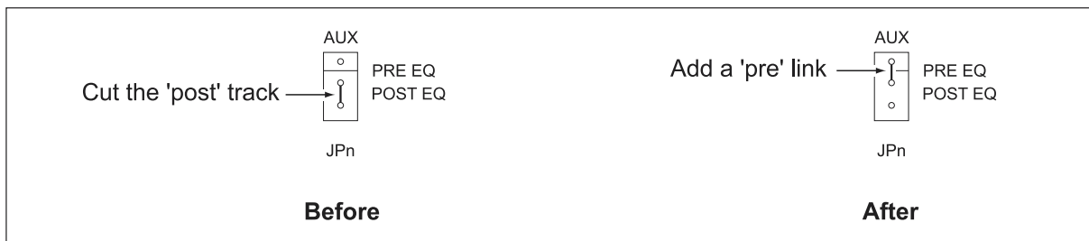
Fig. 10.1: Aux send > pre-EQ modification on mono channels
