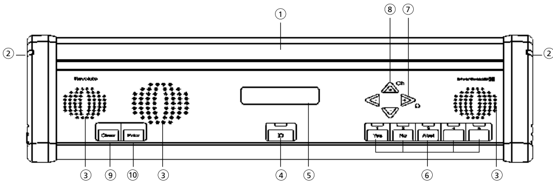
Front view - MCS-D 3173 chairman station
