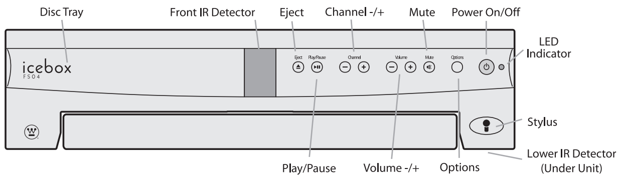
FIGURE 7. Front Panel of iCEBOX FlipScreen
