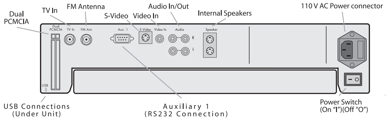
FIGURE 5. Rear Panel of the iCEBOX FlipScreen
