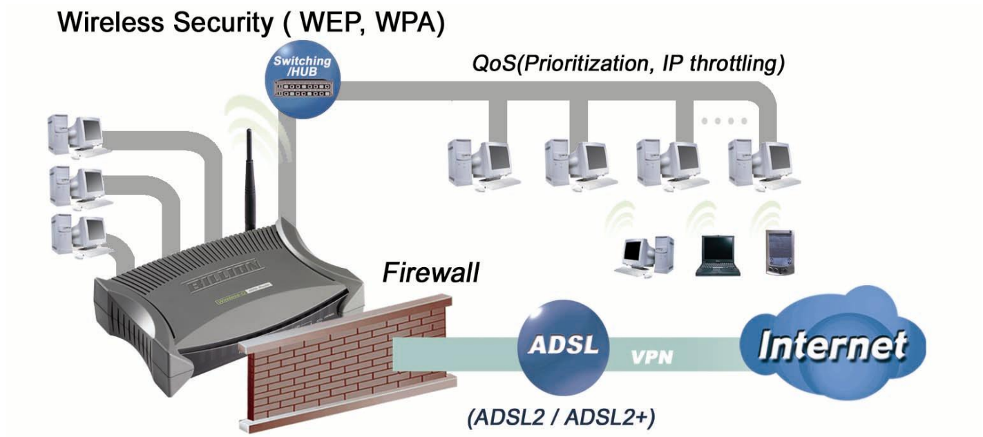
Figure 1.1 Application Diagram of BiPAC 7402G
