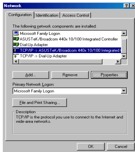
Figure 3.9: TCP / IP
