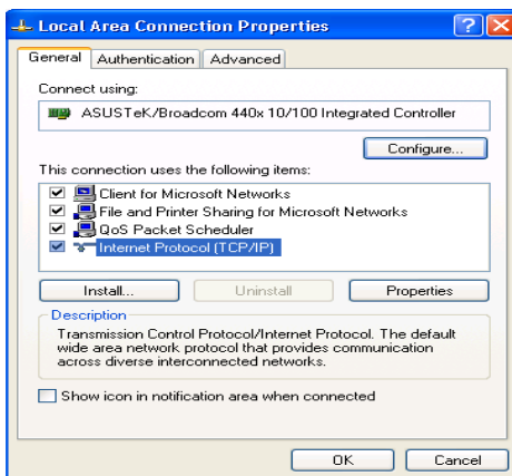
Figure 3.3: TCP / IP
