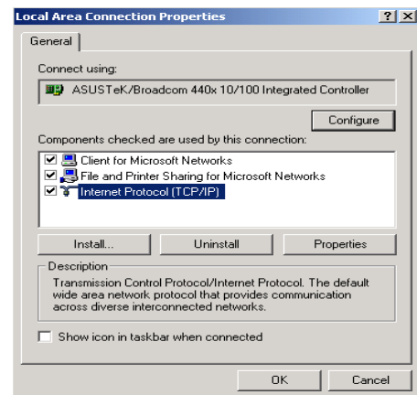
Figure 3.7: TCP / IP
