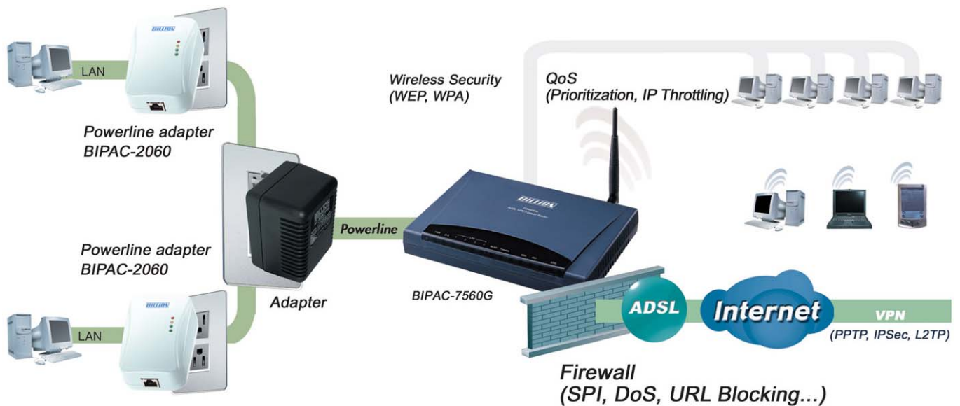
Figure 1.2 Application Diagram of BIPAC-7560G Powerline 802.11g ADSL VPN Firewall Router
