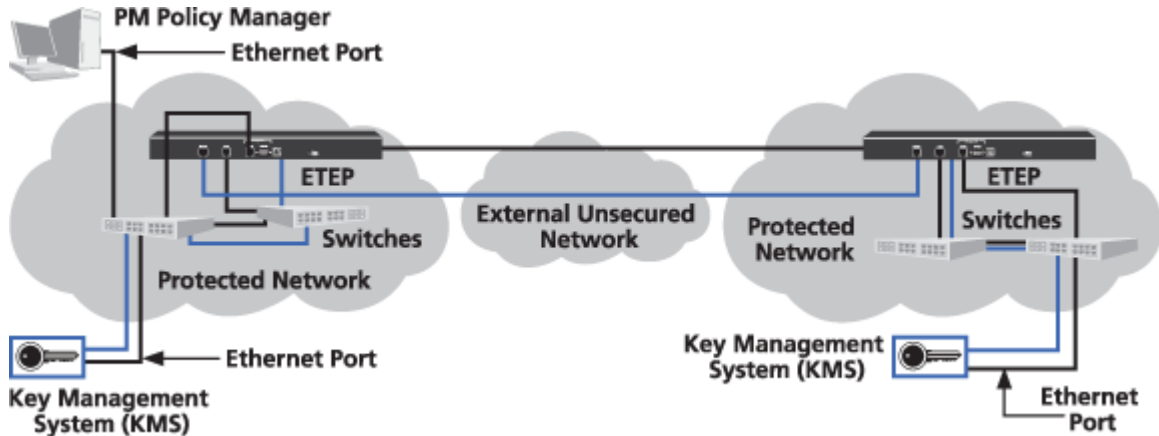
Figure 10 In-line management of ETKMSs located on different IP networks
