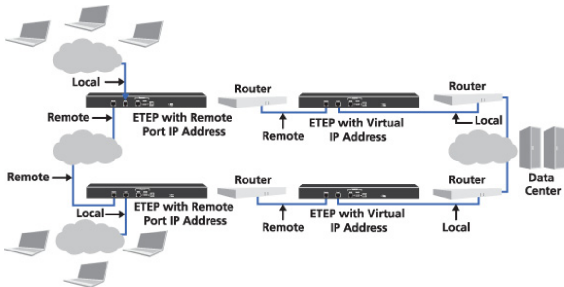
Figure 14 Using remote IP and virtual IP addresses to obscure the source address of the original packet
