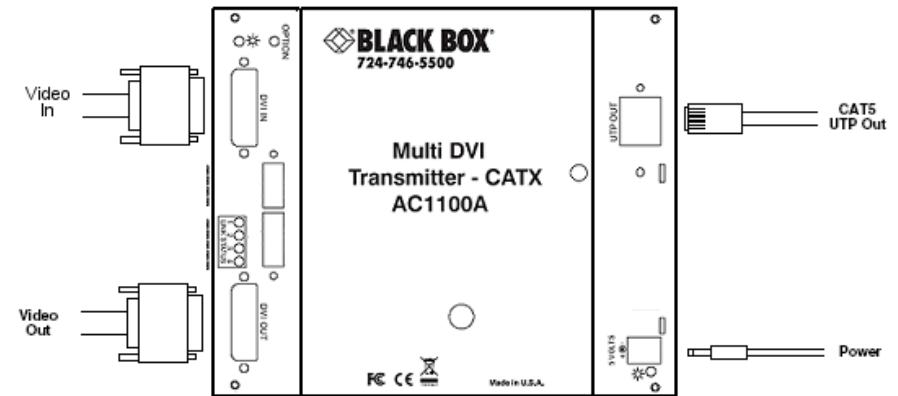
Figure 3-1. Transmitter connections on the AC1100A.
