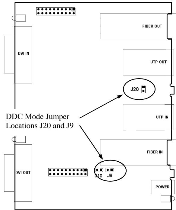
Figure D-1. Jumper locations to change DDC Mode.
