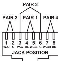
Figure A-2. RJ-45 jack.
