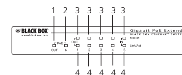
Figure 2-3. LPR1131 front panel.
