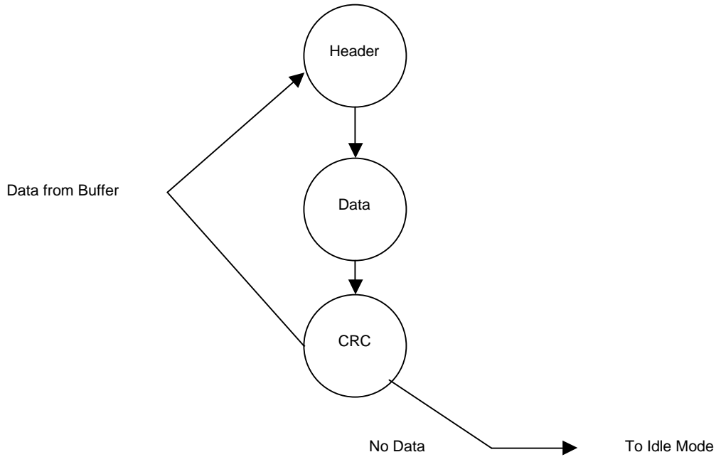
Figure 2b – Transmit Mode Description
