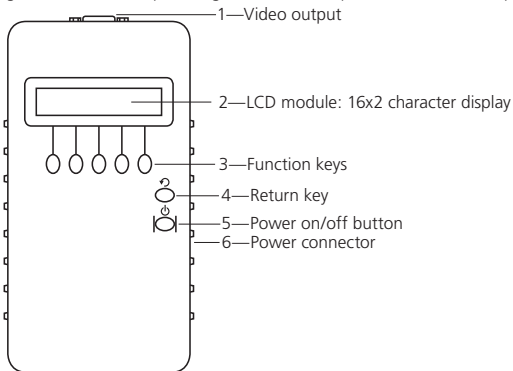
Figure 2-1. Front panel.
