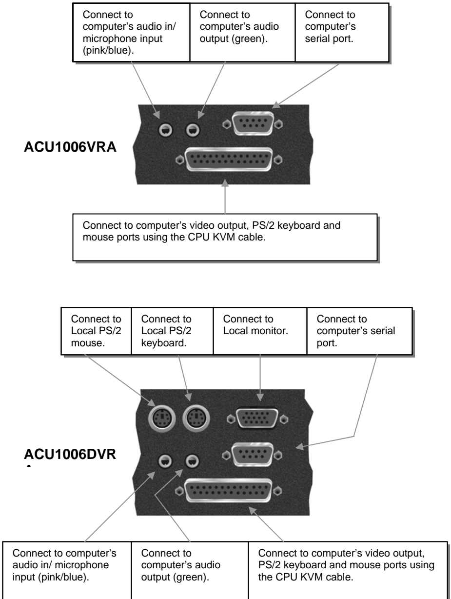
Figure 4 Audio/Serial Hub Port - rear view
