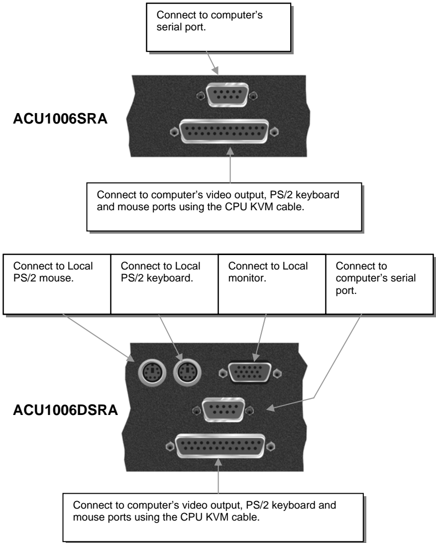
Figure 3 Serial Hub Port - rear view
