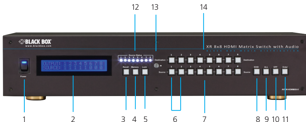
Figure 2-1. Front panel.
