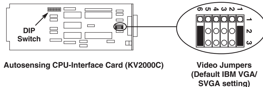
Figure 4-1. The CPU-Interface Card's video jumpers.
