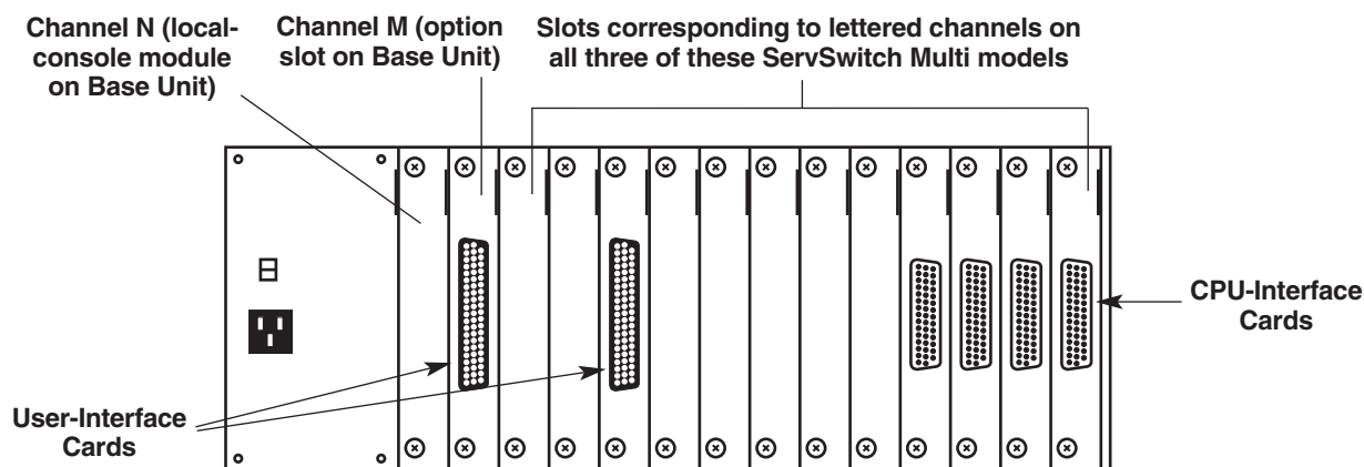
Figure A-1. The rear panel of a ServSwitch Multi Base Unit, EXP, or SB with Cards installed.
