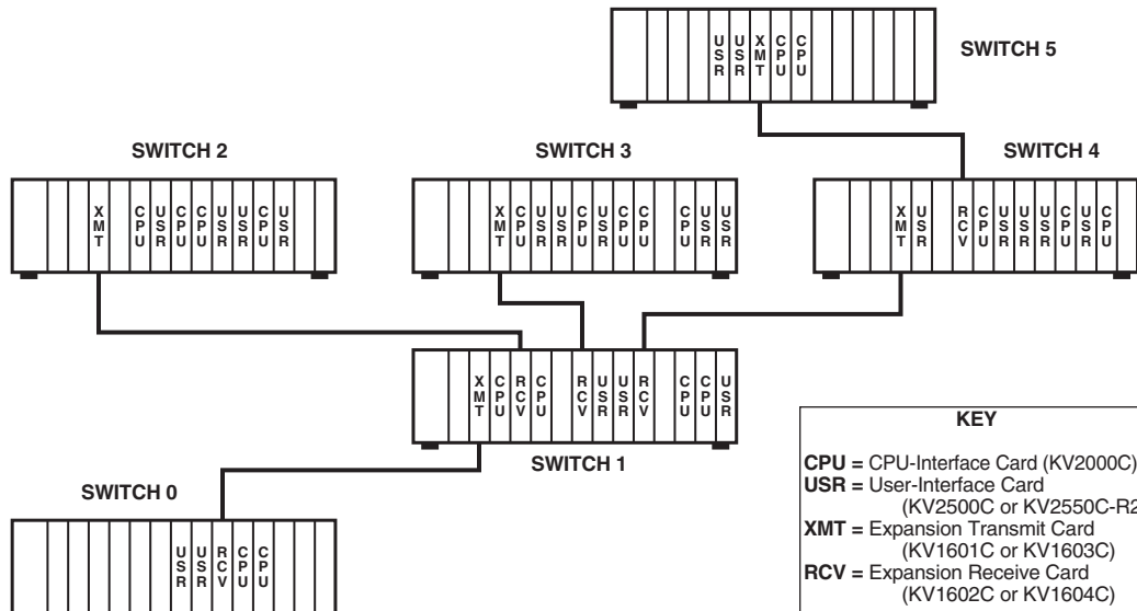
Figure 6-4. A hybrid expanded configuration.
