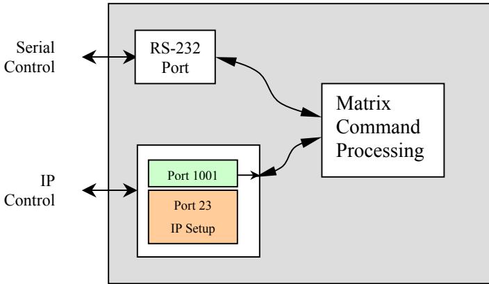
Figure 14 – Control Block Diagram
