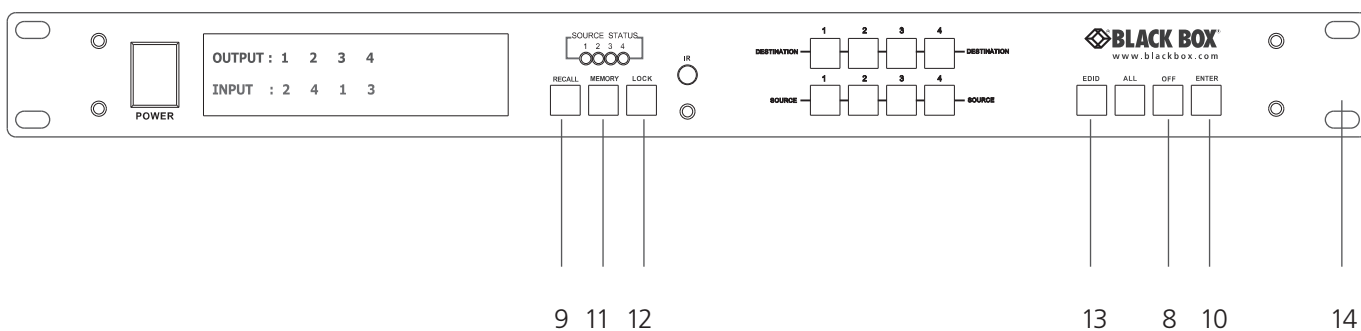
Figure 2-2. Front-panel diagram #2.
