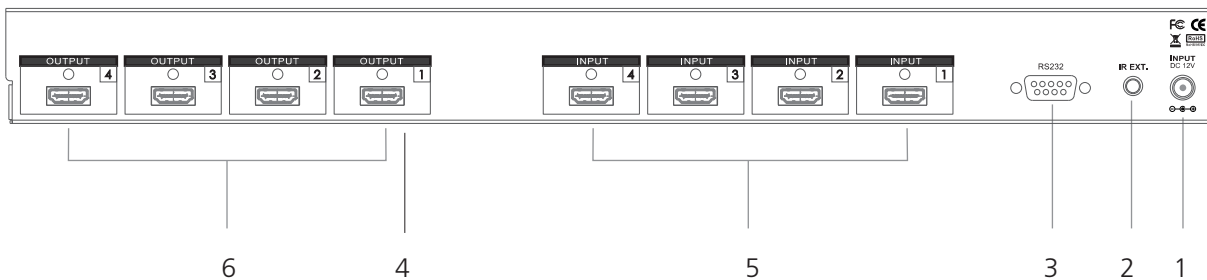
Figure 2-3. Rear panel.
