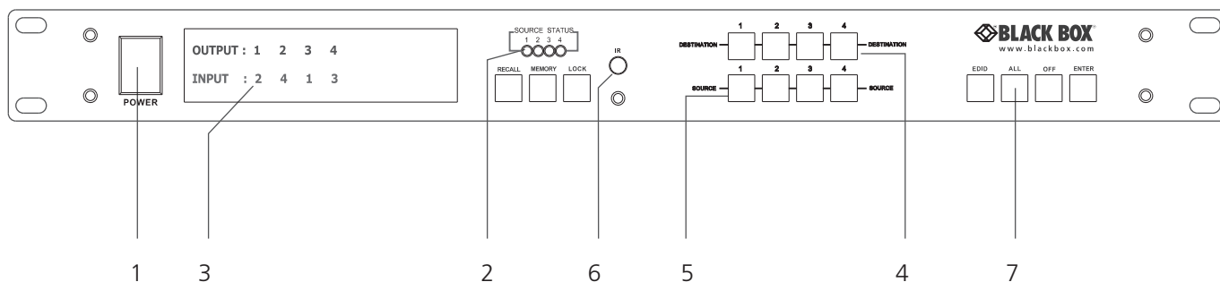
Figure 2-1. Front-panel diagram #1.
