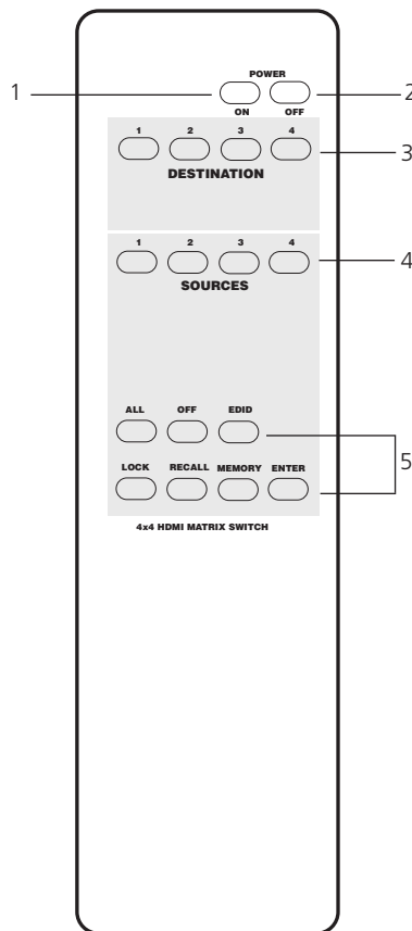
Figure 4-1. IR remote.
