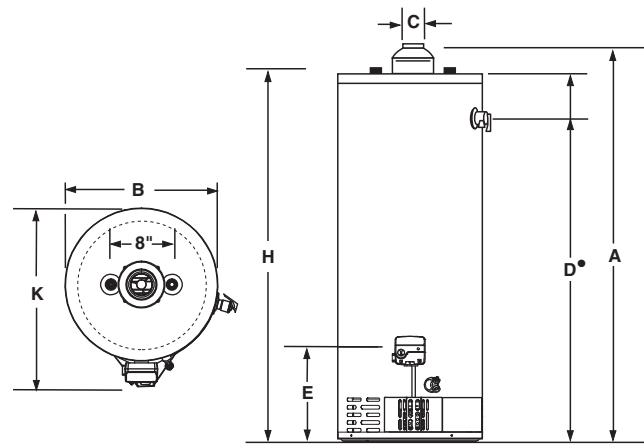
• Optional T&P Location Dimension "D" dimension listed as side/top.
