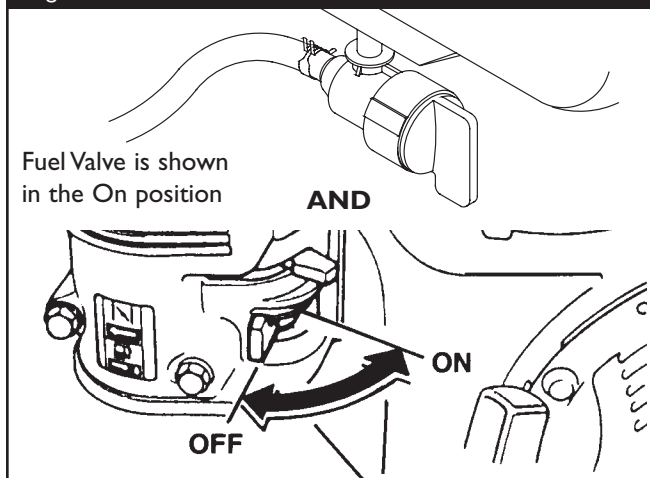
Figure 4 — Fuel Valves
