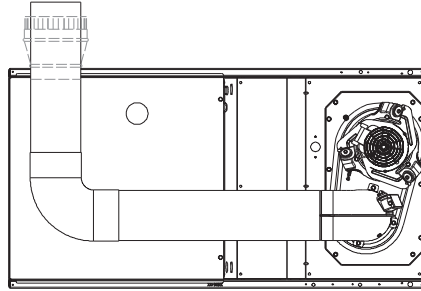
SEE NOTES: 1,2,4,5,7,8,9 HORIZONTAL RIGHT A02070
