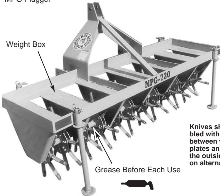
Figure 2 MPG Plugger
