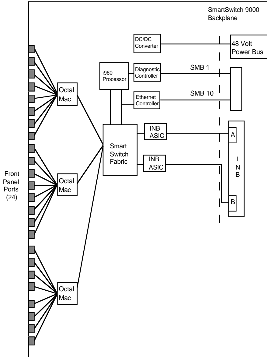
Figure 3-1. Block Diagram
