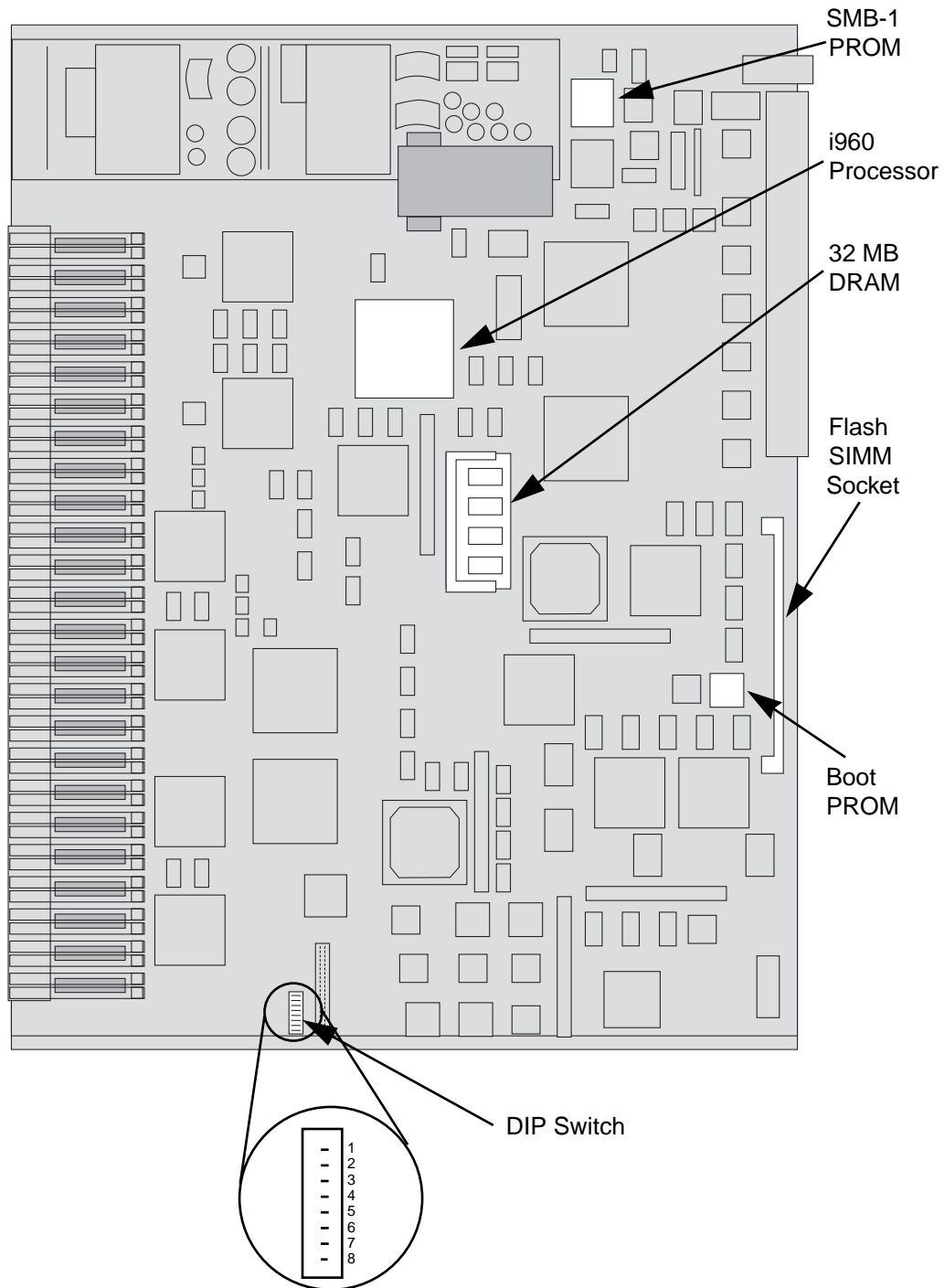
Figure 2-1. User-Accessible Components
