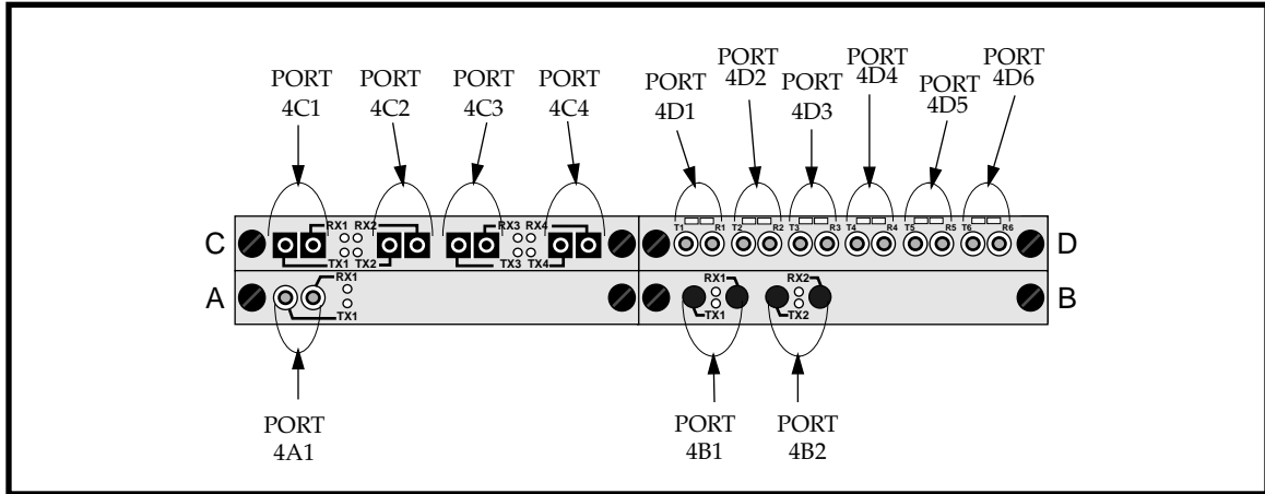
Figure 3.6 - Network Module Port Numbering
