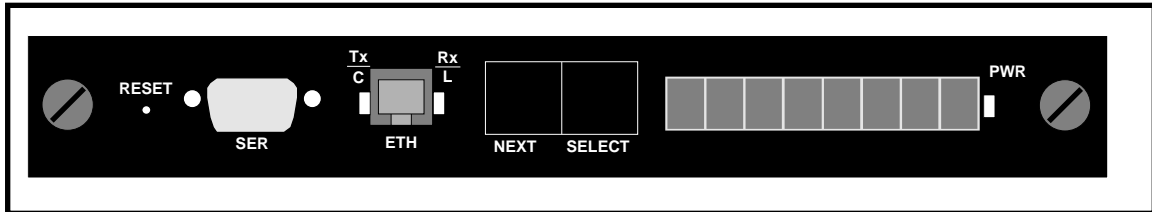
Figure 3.4 - i960 Switch Control Processor Front Panel
