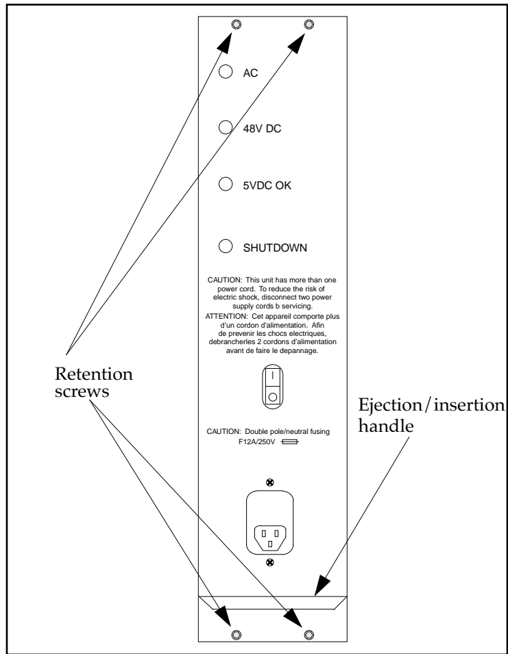
Figure 3.7 - Model A SFCS-1000 AC Power Supply
