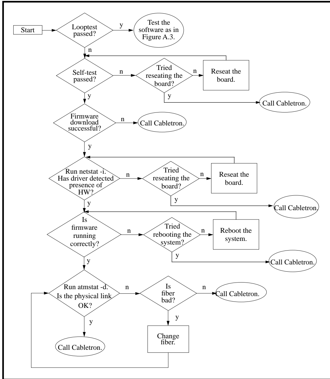
Figure A.1 - Adapter Hardware Troubleshooting Flowchart
