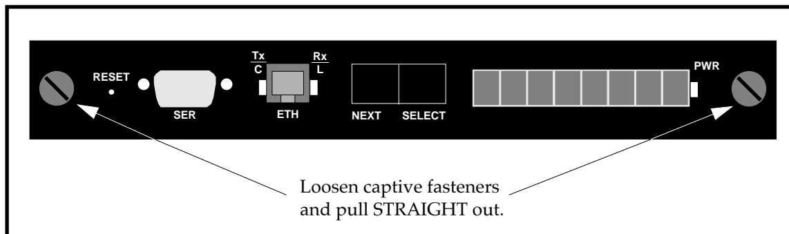
Figure 5.4 - Removal of an SCP
