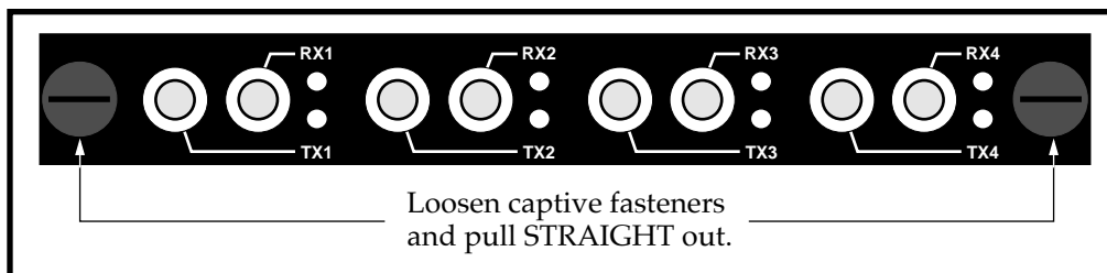
Figure 5.1 - Removal of Network Modules
