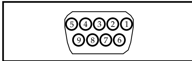
Figure 3.5 - RS-232 Serial Port Pinouts
