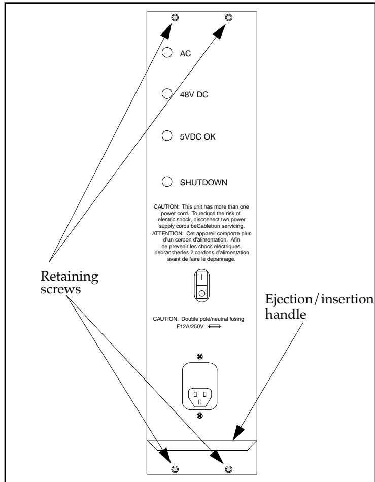
Figure 5.2 - Model A SFCS-1000 AC Power Supply
