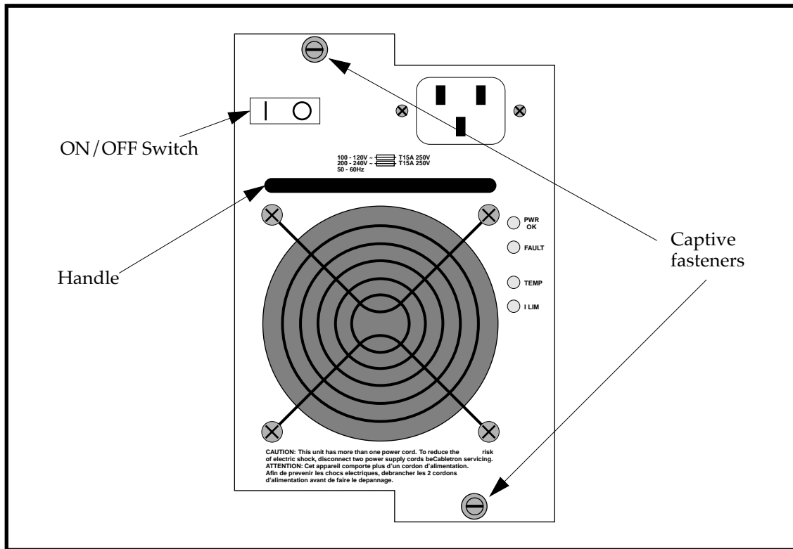
Figure 5.3 - Model B SFCS-1000 AC Power Supply
