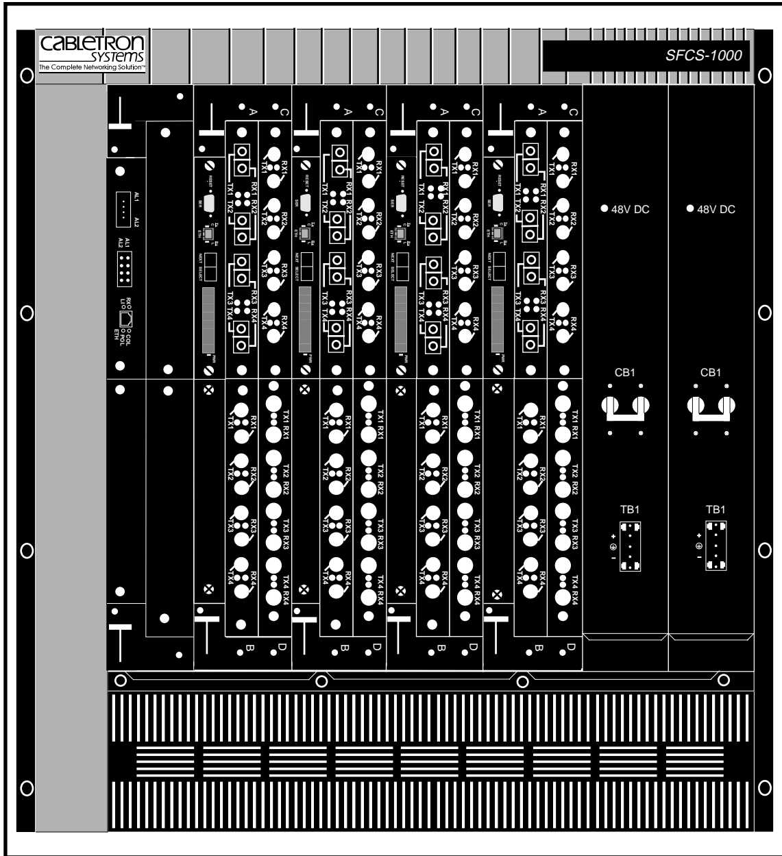
Figure 3.3 - SFCS-1000 Switch Configuration
