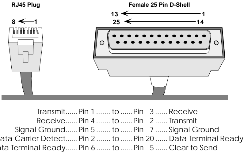
Figure 2-2. RJ45 to DB25 Connector Pinout
