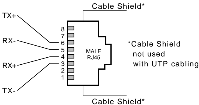
Figure 2-1. TCU pinouts
