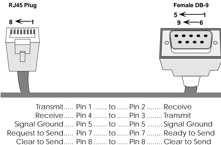
Figure 2-3. RJ45 to DB9 Connector Pinout
