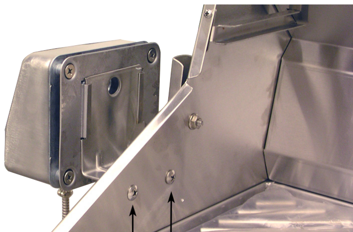
Attachment screws for rotis motor
